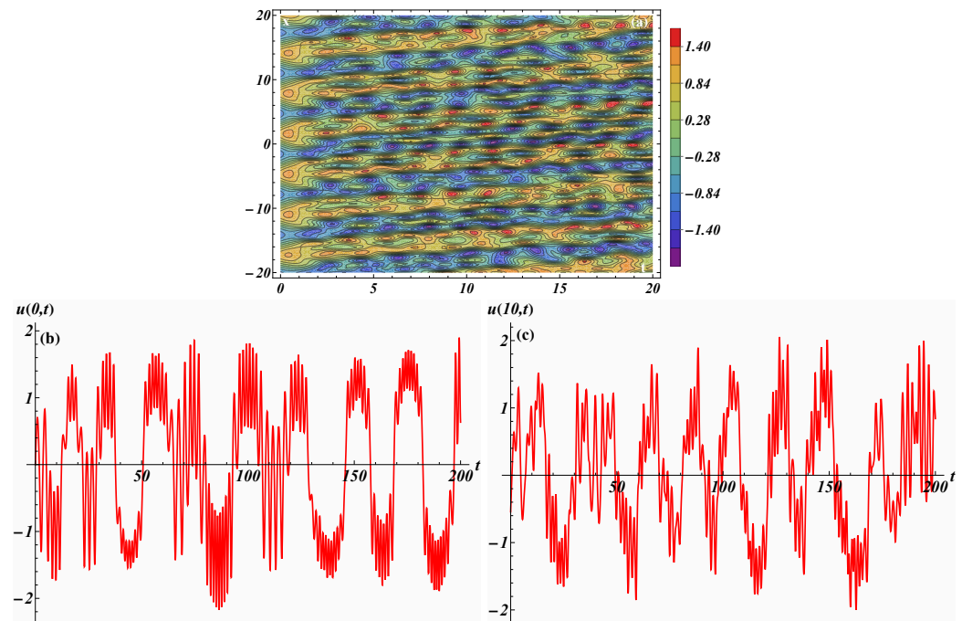
Figure 5. Classical solutions to the initial-boundary value problem for the n = 4 rotated modified KdV equation with boundary value functions (126) in panel (a) and selected timelines for fixed values of x in panels (b,c).
