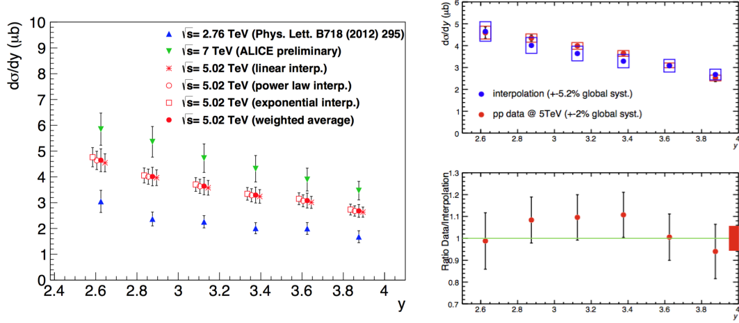
Figure 2.6: Left: Inclusive J/\psi differential cross-section as a function of rapidity at \sqrt{s}=2.76 and 7 TeV and interpolated cross-section at \sqrt{s}=5.02 TeV obtained with the three interpolation functions as well as for the average values. Right: Inclusive J/\psi cross-section as a function of rapidity at \sqrt{s}=5.02 TeV and compared to the interpolated cross-section.
