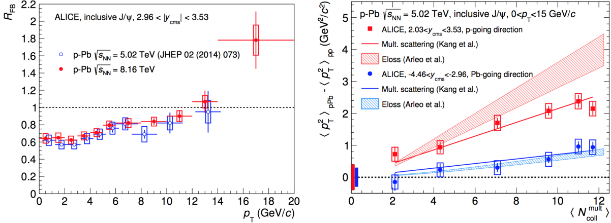
Figure 2.15: Left: forward-to-backward ratio of inclusive J/ψ in pPb collisions at \sqrt{s_{NN}} = 5.02 and 8.16 TeV [74, 77] as a function of p_T . Right: p_T broadening as a function of the number of binary collisions at \sqrt{s_{NN}} = 5.02 TeV [83].
