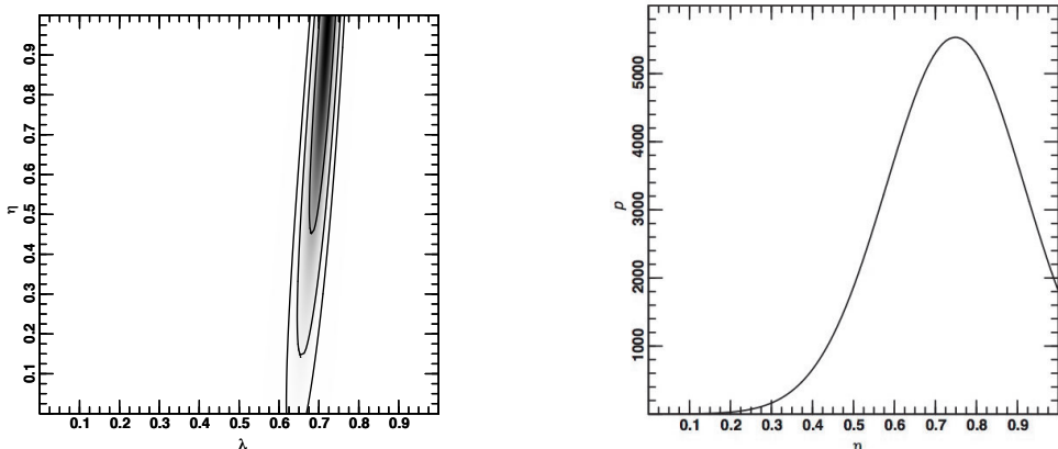
Figure 2 – Left : Two-dimensional PD for k = 0 . Right : One-dimensional PD for the concordance model.
