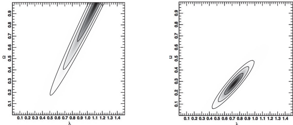
Figure 1 – Left : Two-dimensional probability distribution (PD) for \eta = 0 . Right : The same for \eta = 1 .
