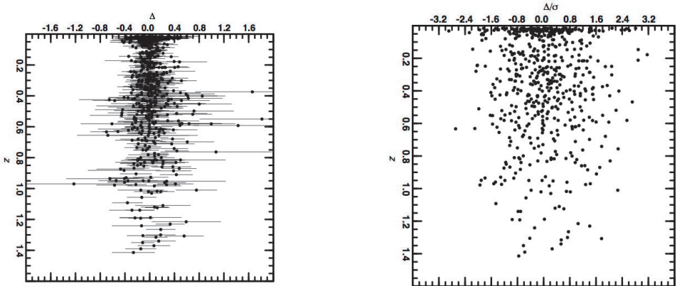
Figure 3 – Left : Residuals (points) and observational uncertainties (error bars). Right : Quotients of residuals and observational uncertainties.
