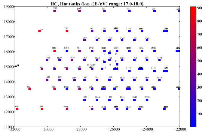
Figure 3.9: Map of the SD in the infill+HEATlet region and their event counts in hybrid with HeCo (color scale). An event is counted only for the stations closest to the shower core. Black squares are Coihueco and HEAT locations.
