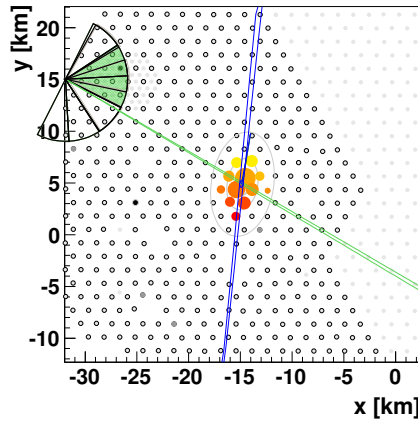
(c) Distribution of an SD Event.
