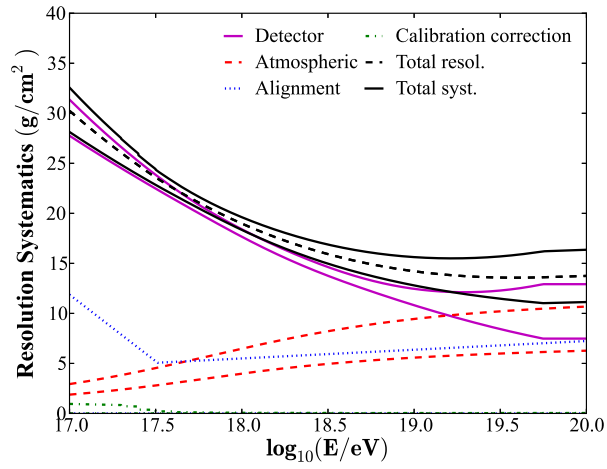
(c) Resolutions and its systematic.
