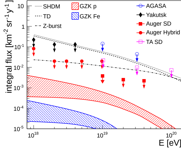
Figure 2.3: Integral limits on the flux of photons at 95 % CL from air shower experiments, compared to the predictions from top-down models and GZK effects. Experimental data are shown from AGASA, Yakutsk, Auger and TA. Top-down scenarios are from the super-heavy DM (SHDM), topological defect (TD) and Z-Bursts. Photons from the GZK effect (Eq. (2.4)) are predicted for the energy loss from protons and irons. From [23].
