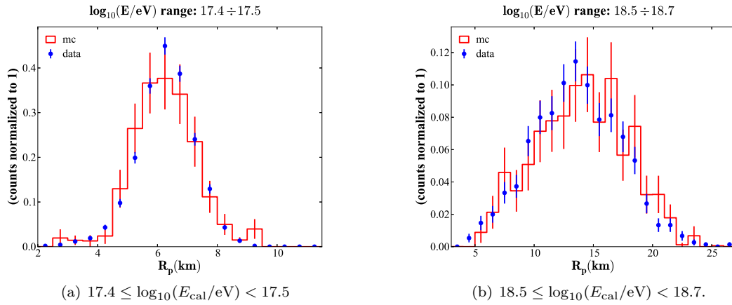
Figure 5.6: Examples of the R_p comparison between data (blue) and MC (red) in two different \log_{10}(E_{\text{cal}}/\text{eV}) bins.
