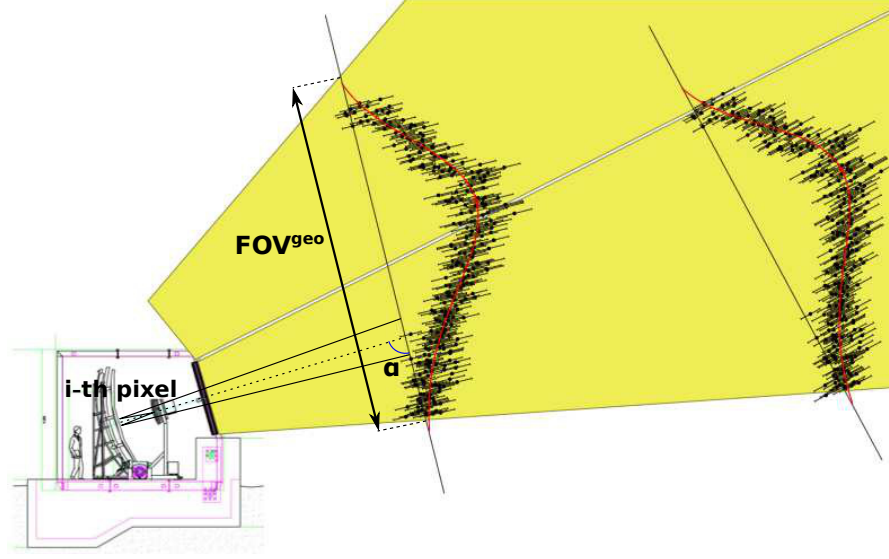
Figure 3.5: Downward and upward fields of view that compound the virtual location HeCo, and how longitudinal shower profiles are seen from the different FoV. \text{FOV}^{\text{geo}} is the geometrical FoV of HeCo. Picture modified from [57]
