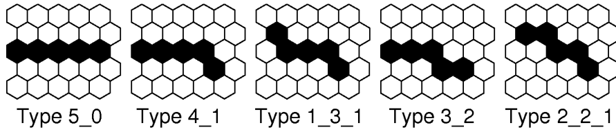
Figure 3.6: Patterns searched by the SLT (from [54]).
