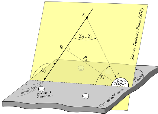
(a) Scheme of the shower geometry. Index i refers to the i -th pixel.
