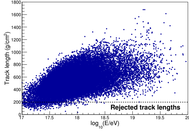
Figure 4.5: Scatter plot of the track length as a function of \log_{10}(E/\text{eV}) . The dashed line is the level of the Minimum track length cut.
