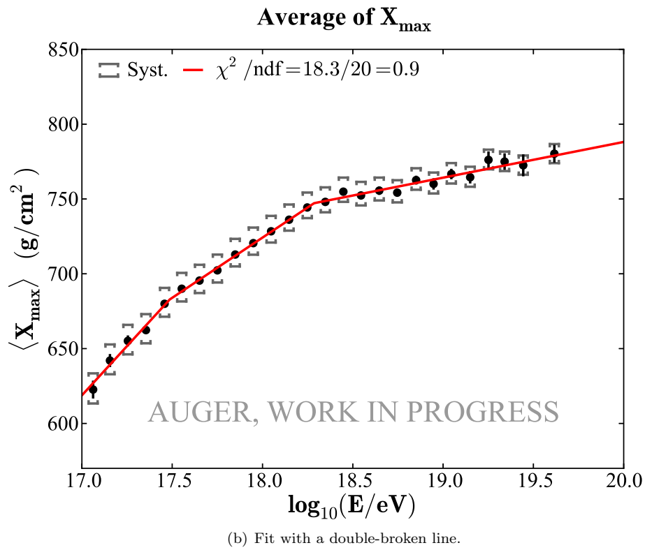
Figure 7.3: \langle X_{\max} \rangle measurement and the fit (red solid line) of its elongation rate.
