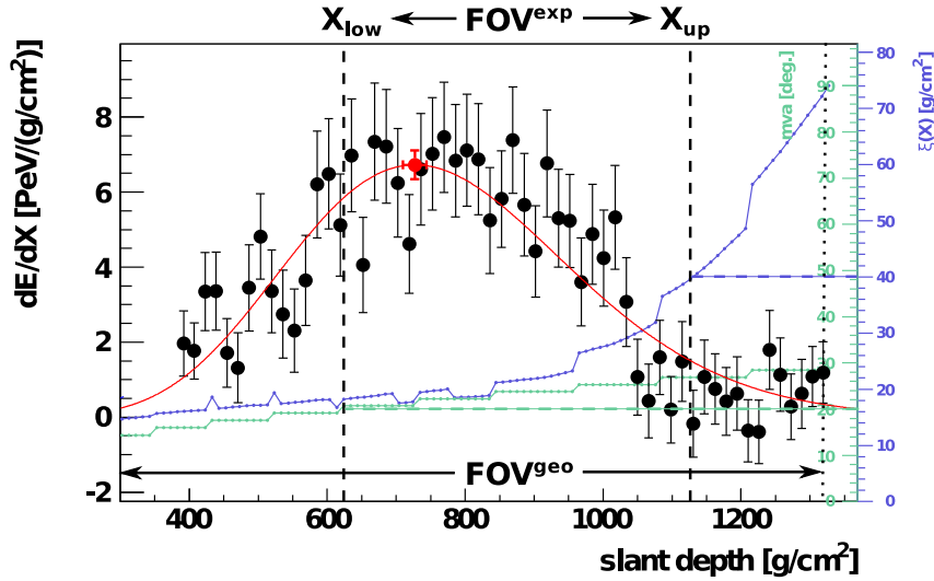
Figure 4.9: Example of geometrical ( \text{FOV}^{\text{geo}} ) and Expected FoV ( \text{FOV}^{\text{exp}} ) delimited by \xi (blue markers) and estimated mva (green markers) limits. The black markers are the deposited energy dE/dX in the telescope. The red line is the Gaisser-Hillas profile and the red dot X_{\text{max}} .
