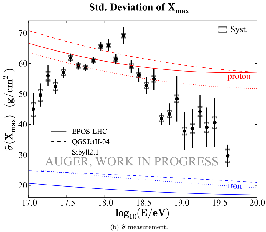
Figure 7.2: Results for the moments of the X_{\max} distribution. The values from air shower simulations using the hadronic interaction models (EPOS-LHC, QGSJetII-04, Sibyll2.1) are shown for pure proton and pure iron compositions.
