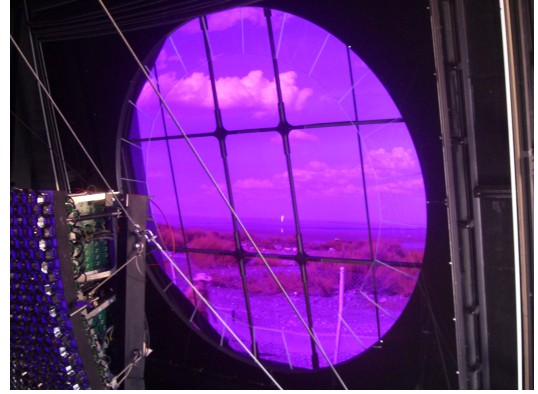
(b) UV filter and corrector ring at the bay aperture.
