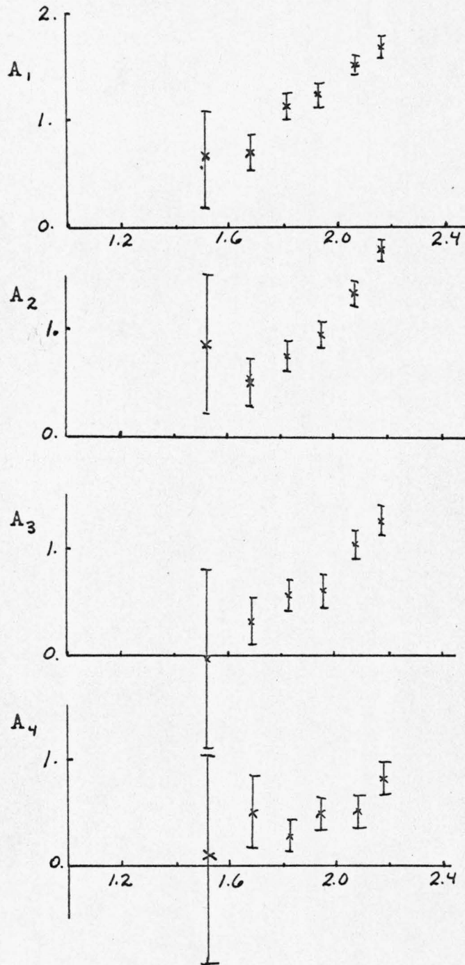
Figure 21. Legendre Expansion Coefficients for the Reaction K^*p \rightarrow K^*0 \Delta^{++} .
