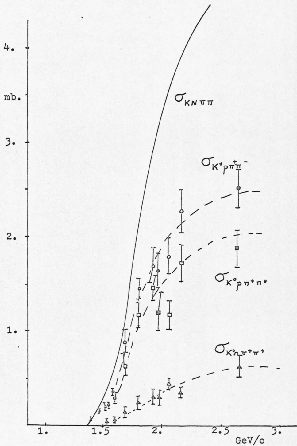
Figure 6. Two Pion Production Cross-sections Open symbols refer to this experiment, solid to reference 11 .
