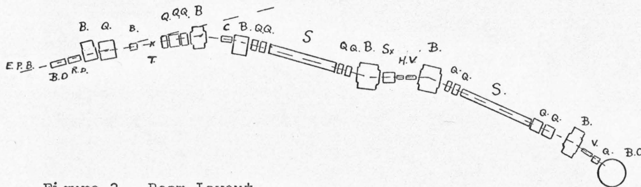
Figure 3. Beam Layout
