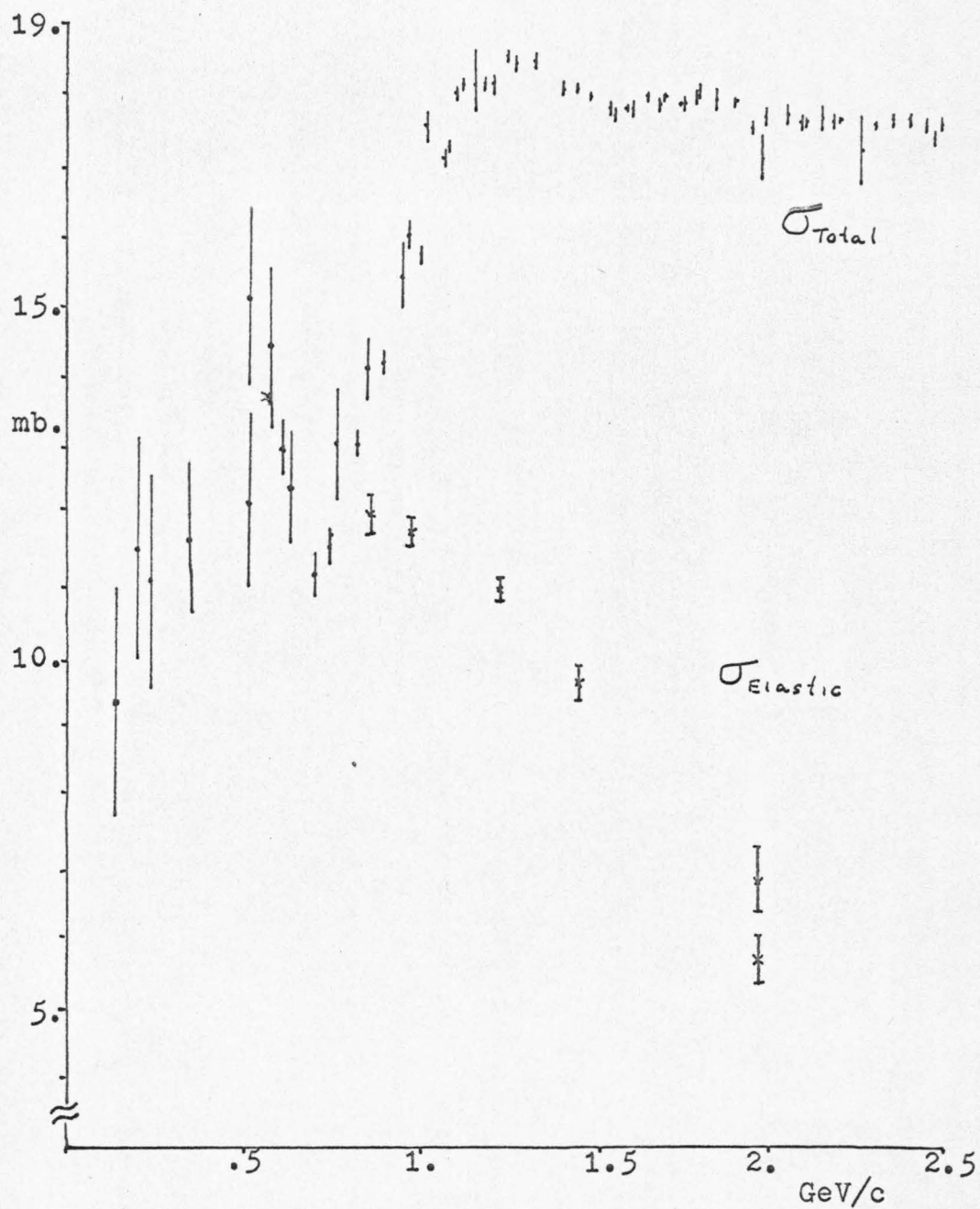
Figure 1. K^+p Elastic and Total Cross-sections
