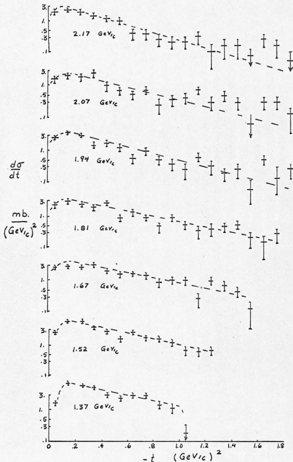
Figure 18. Differential Cross-section for K^+p \rightarrow K^{*+}p The curves are to guide the eye.
