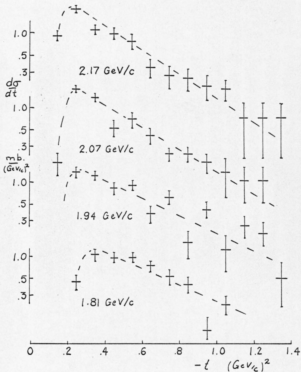
Figure 22. Differential Cross-sections for K^+p \rightarrow K^*\Delta . The curves are to aid the eye.
