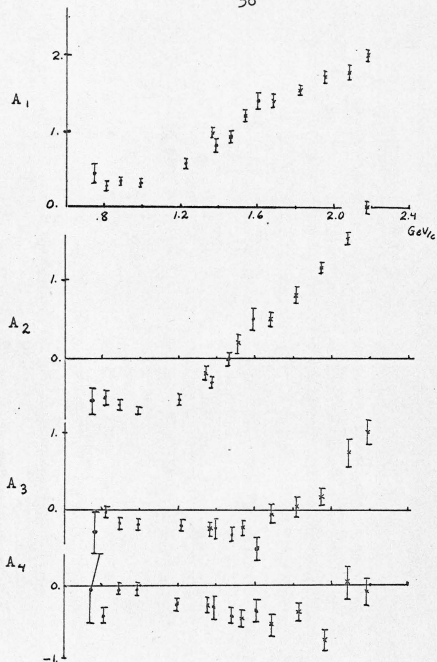
Figure 13. Legendre Expansion Coefficients for the Reaction K^+p \rightarrow K^0 \Delta^{++} .
