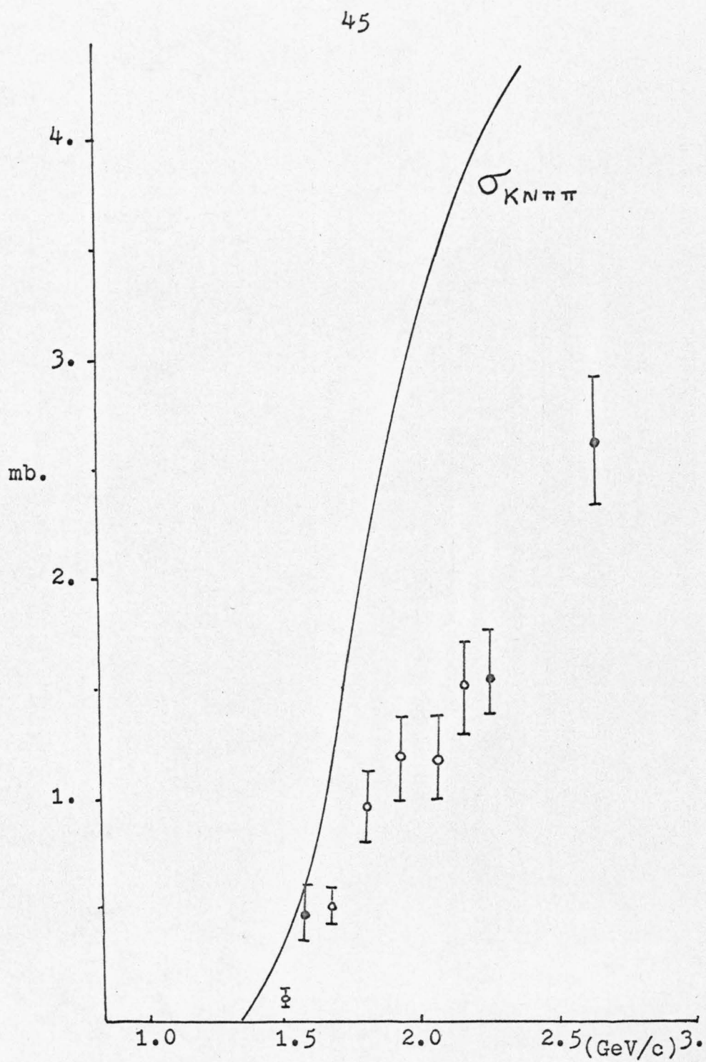
Figure 10. Cross-sections for K^*\Delta Production. Open symbols refer to this experiment, solid to reference 11.
