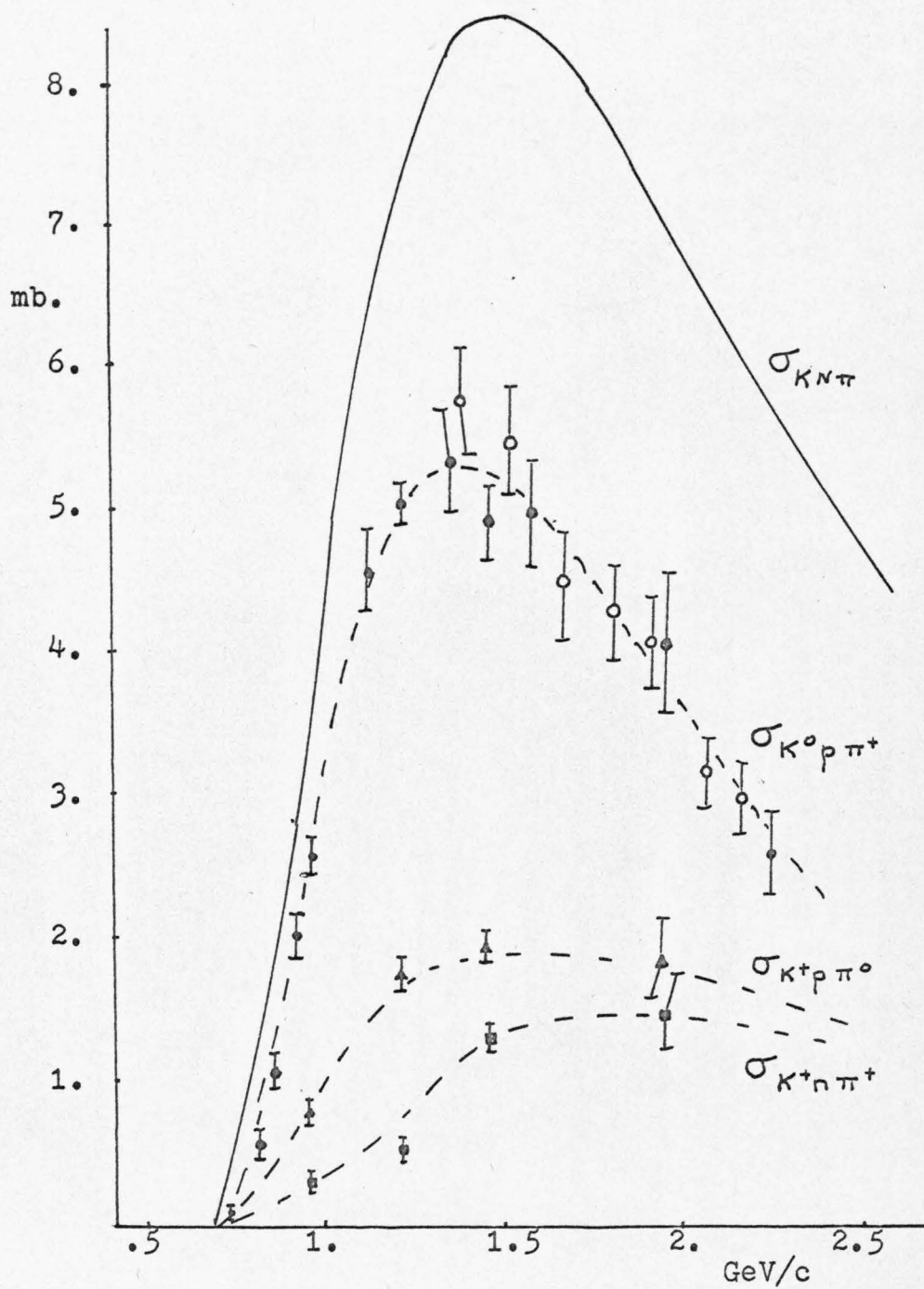
Figure 5. Single Pion Production Cross-sections The open symbols refer to this experiment, the solid to reference 10 .
