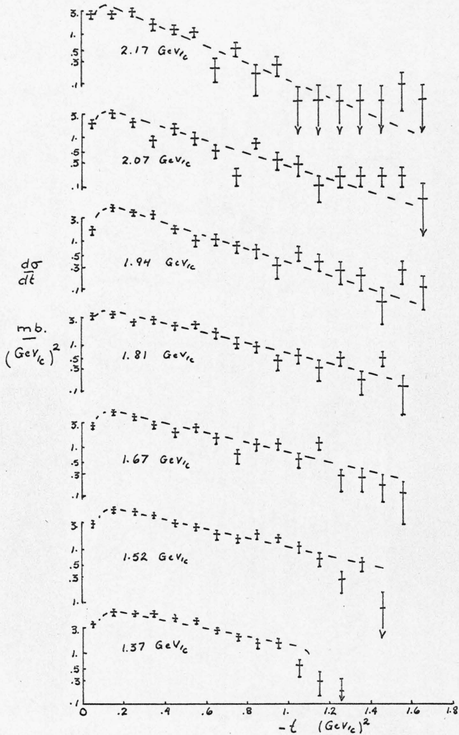
Figure 14. Differential Cross-sections for K^+p \rightarrow K^0\Delta^{++} . The curves are to aid the eye.
