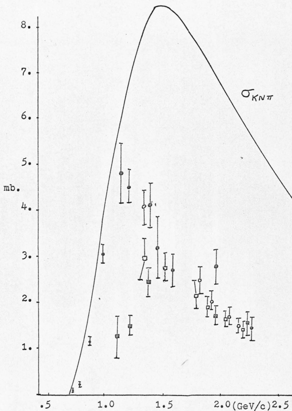
Figure 8. Cross-sections for K\Delta and K^*N Production. Data for K\Delta shown by \square and \circ ; K^*N by \blacksquare and \bullet . The open symbols refer to this experiment, solid to reference 10.
