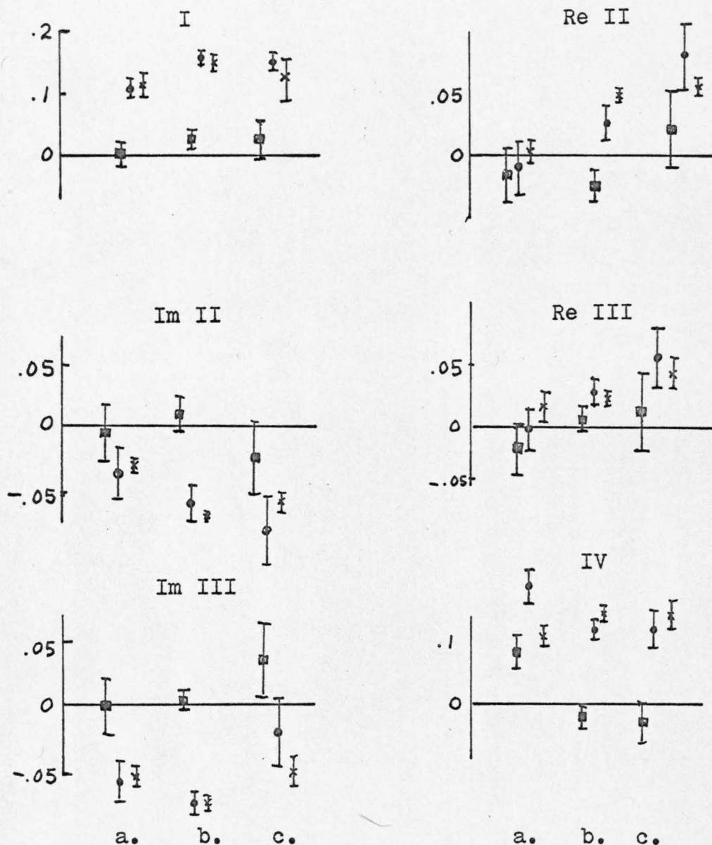
Figure 25. Test of Quark Scattering Relations for three momenta. a) 1.8 - 2.2 GeV/c, this expt. b) 2.5 - 3.2 GeV/c, ref. 17. c) 5.0 GeV/c, ref. 17. The figure shows the difference \bar{F} , left side \bar{F} , and right side \bar{F} .
