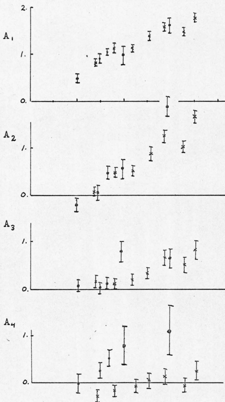
Figure 17. Legendre Expansion Coefficients for the Reaction K^+p \rightarrow K^{*+}p .
