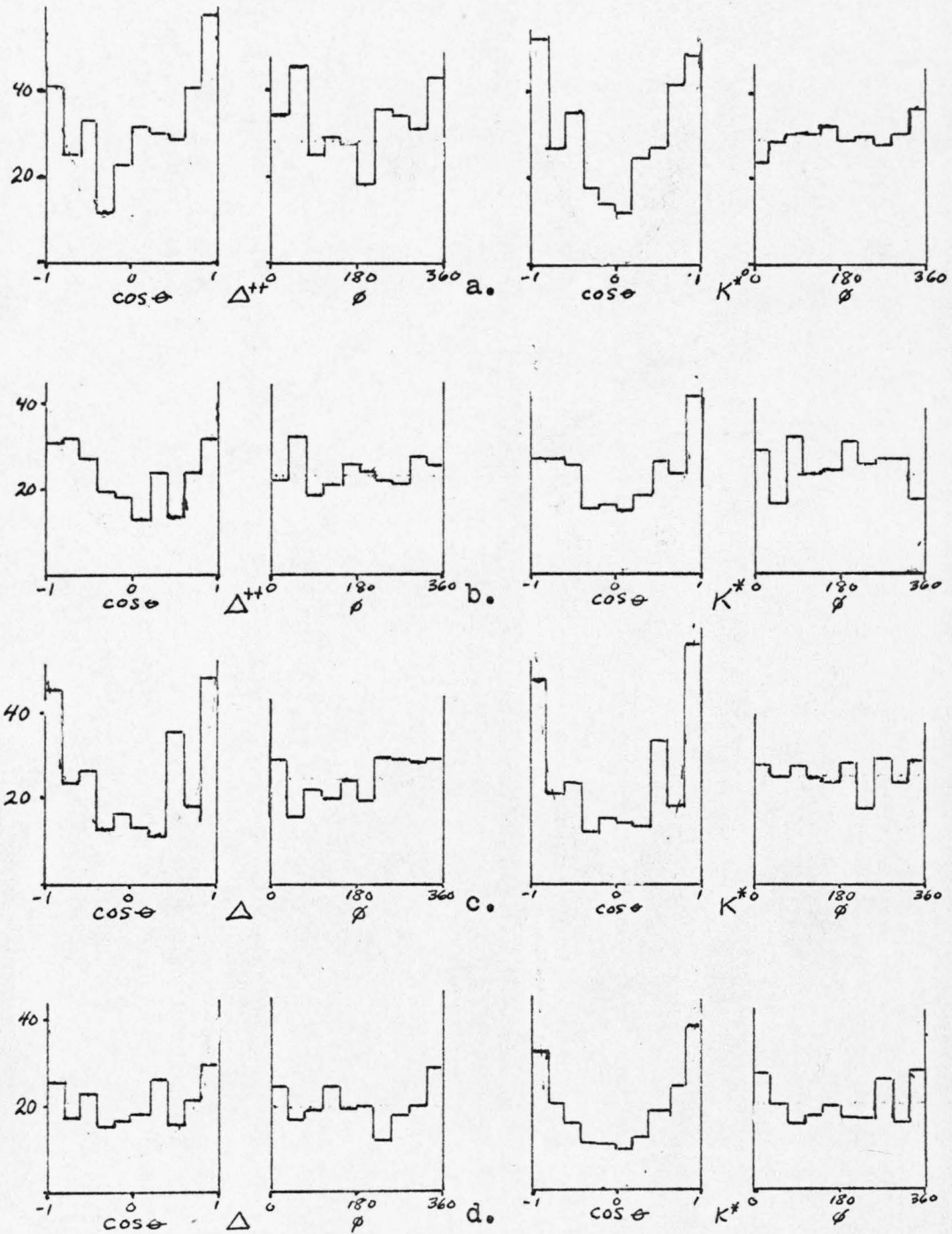
Figure 23. Decay Angular Distributions for the Reaction K^+p \rightarrow K^{*0} \Delta^{++} at four momenta: a. 2.17 GeV/c, b. 2.07 GeV/c, c. 1.94 GeV/c, d. 1.81 GeV/c.
