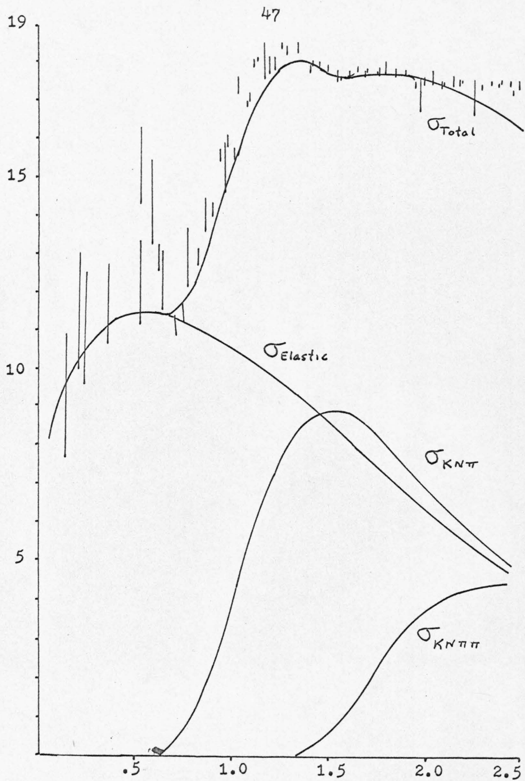
Figure 11. K^+p Partial Cross-sections.
