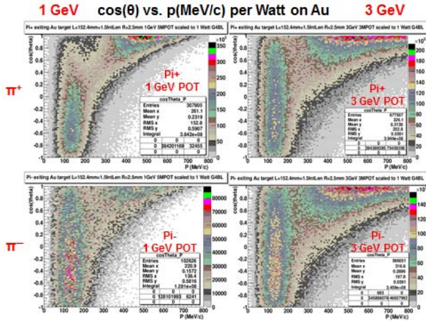
Figure 5: The fluxes of \pi^+ 's (upper) and \pi^- 's (lower) exiting a gold target vs. \cos(\theta) and P(\text{MeV/c}) for protons of 1 GeV (left plots) and 3 GeV (right plots).
