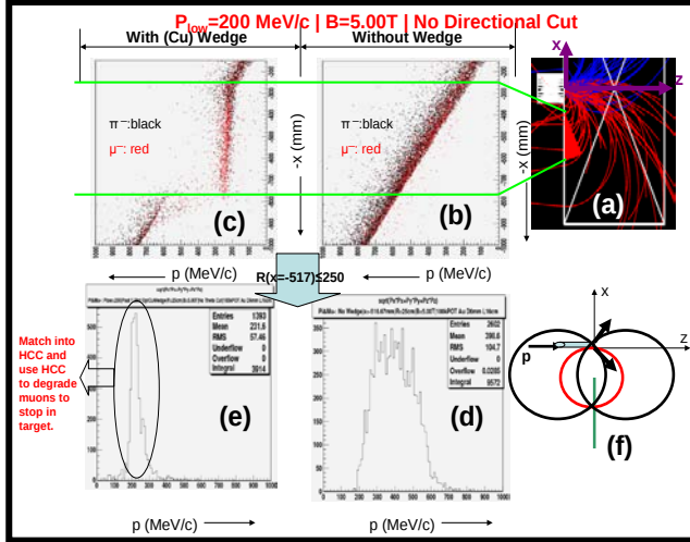
Figure 2: The Dipole/Wedge configuration to produce a 200 MeV/c pion beam in a dipole field of 5 T. (a) Top view of pions and muons in the Dipole/Wedge. Negatively (positively) charged particles are red (blue). (b) and (c) Correlation between momenta and horizontal exit position from the dipole for \pi^- and \mu^- without and with a wedge, respectively. (d) and (e) Momentum projection from (b) and (c), respectively. Note direction reversal of momentum plot for (d) and (e). (f) Cartoon explaining momentum asymmetry in (b). Pions with a non-zero production angle must have a higher momentum in order to reach the same horizontal position at the wedge.
