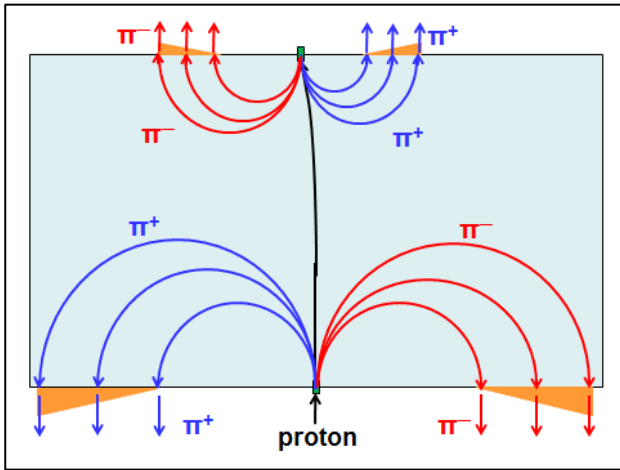
Figure 3: Layout of single dipole with two targets and four wedges to produce four monoenergetic pion beams from a single proton beam.
