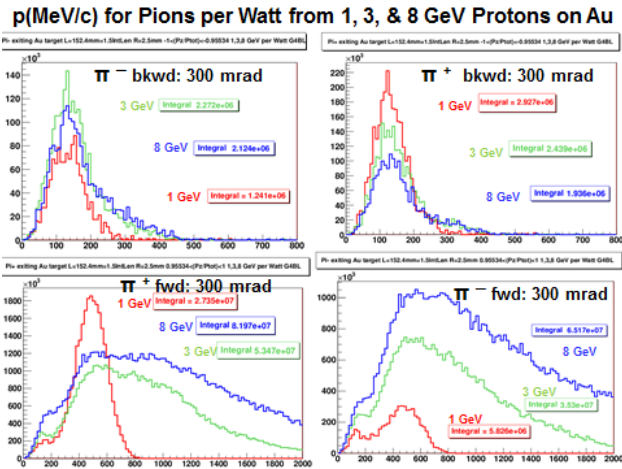
Figure 3: Momentum spectra (MeV/c) of \pi^+ 's and \pi^- 's traveling forward (within 300 mrad) or backward ( <300 mrad), produced by 1, 3, and 8 GeV protons. The plots are normalized to 1 Watt of beam power. The placement of the plots (right/left & upper/lower) matches the location of the beams in Figure 3.
