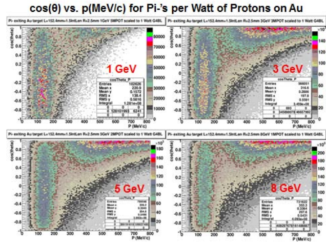
Figure 4: The fluxes of \pi^- 's exiting a gold target vs. \cos(\theta) and P (MeV/c) for protons with kinetic energy 1 GeV (upper left), 3 GeV (upper right), 5 GeV (lower left), and 8 GeV (lower right). Entries in plots are scaled to a beam power of 1 Watt.
