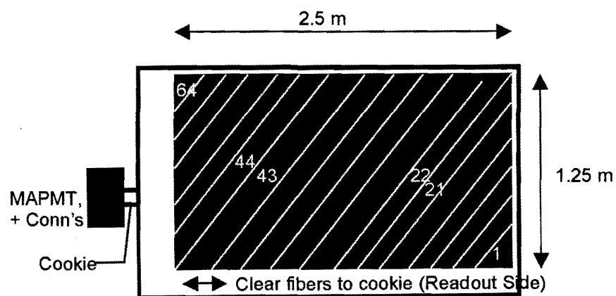
Schematic of Test Module with Single Sided Readout
