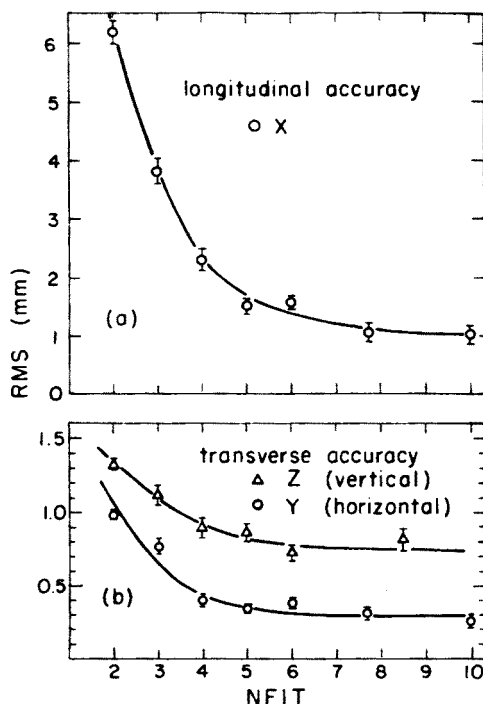
Fig. 5. Vertex prediction accuracy versus the number of tracks entering into the vertex fit; only fits consisting of the same tracks but resulting from independent measurements of an event were compared to estimate the accuracy: (a) location along the beam; (b) location transverse to the beam
