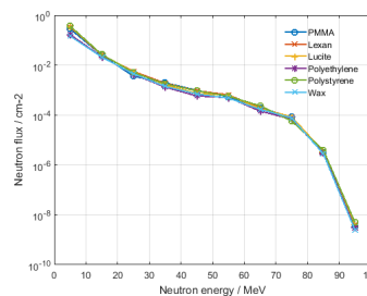
Figure 9: Neutron yield corresponding to different material range shifters.
