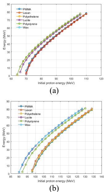
Figure 6: Relationship between the initial energy and the modulated energy(3.5cm(a)/6.5cm(b)).
