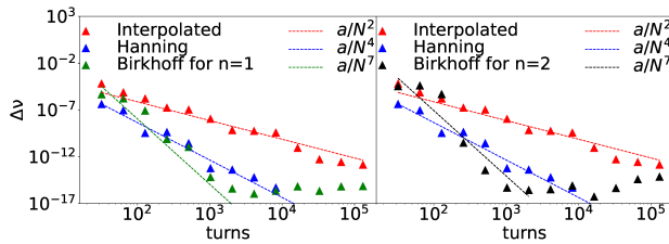
Figure 1: Comparison of the tune error \Delta \nu as a function of the length of the time series N for various methods including the Birkhoff average with n = 1 (left) and n = 2 (right). The improved performance of the method based on Birkhoff average is clearly visible.
