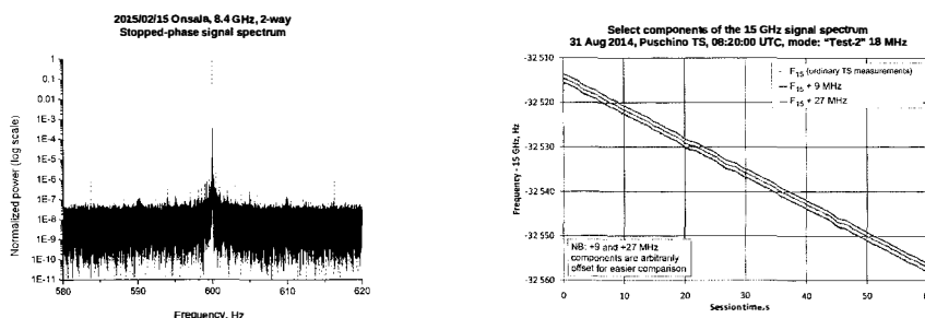
Figure 1 – a) Result of the carrier frequency (8.4 GHz) measurement, b) The time evolution of the carrier (15 GHz) and two sidebands
