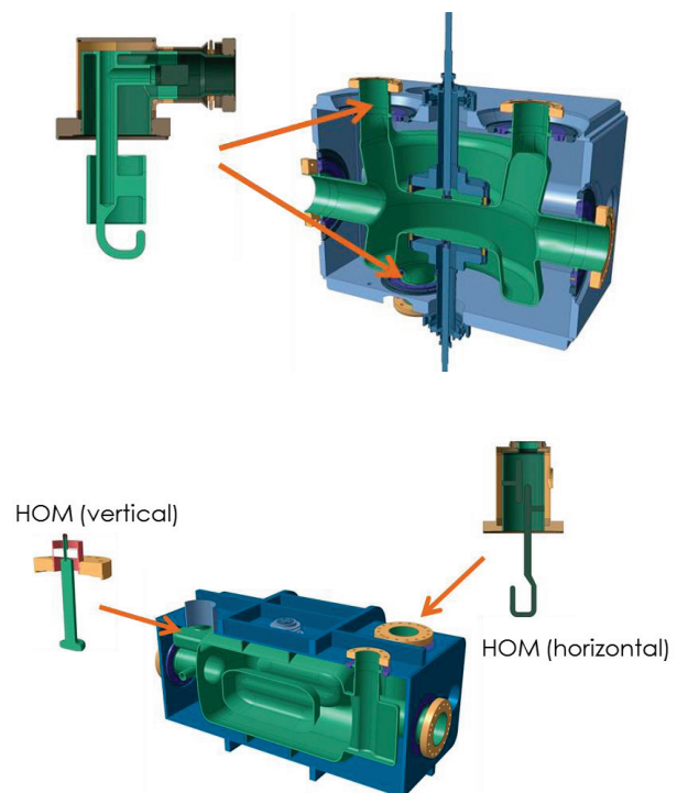
Figure 10: HOM couplers for DQW (top) and RFD (bottom) crab cavities with helium vessel.
