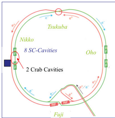
Figure 3: Crab cavity location for KEKB.
