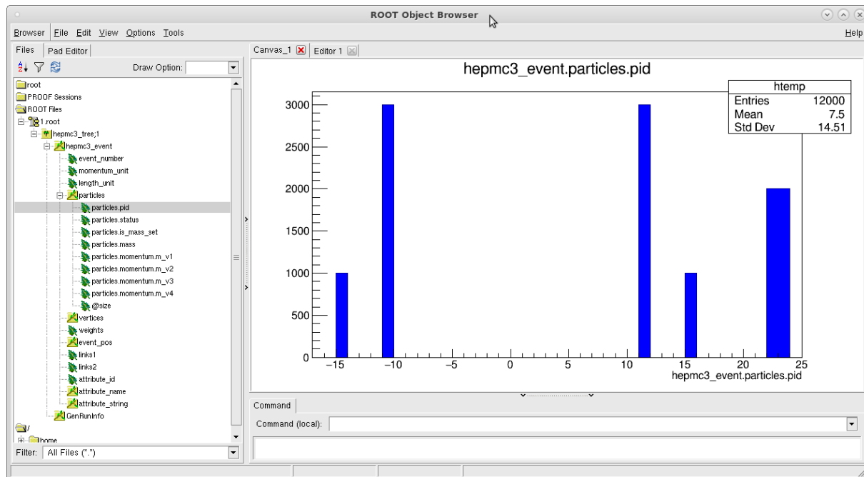
Figure 1. Inspection of e^-e^+ \rightarrow \tau^-\tau^+ events simulated by the Pythia8 [8] Monte Carlo event generator. The file with HepMC3 events (ROOTTree) is explored with the ROOT Object browser without loading of the HepMC3 library.
