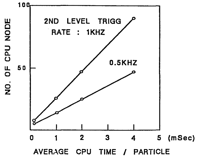
Fig. 12: Number of CPU nodes required for the farm as a function of the CPU speed (msec/particle)
