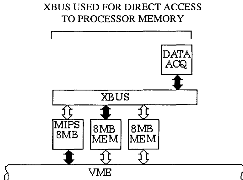
Figure 5. The memory extension bus (XBus) allows direct access into the memory of the ACP MIPS processor board.
