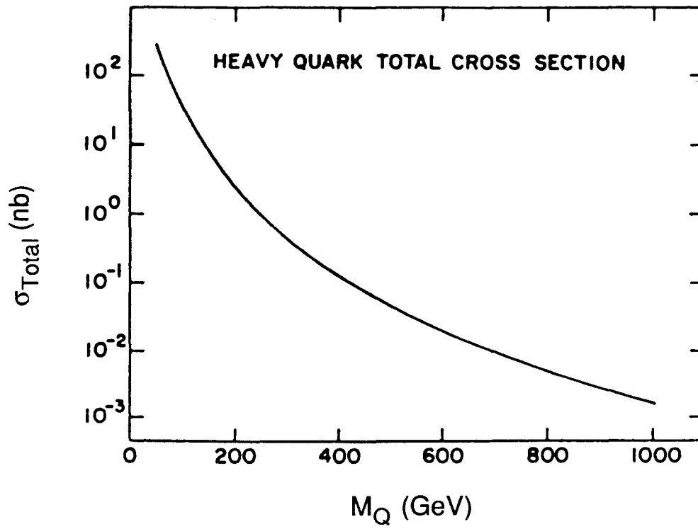
Fig. 7. The total production cross section for new down-like quark pair production at the SSC. Taken from Ref. 9.
