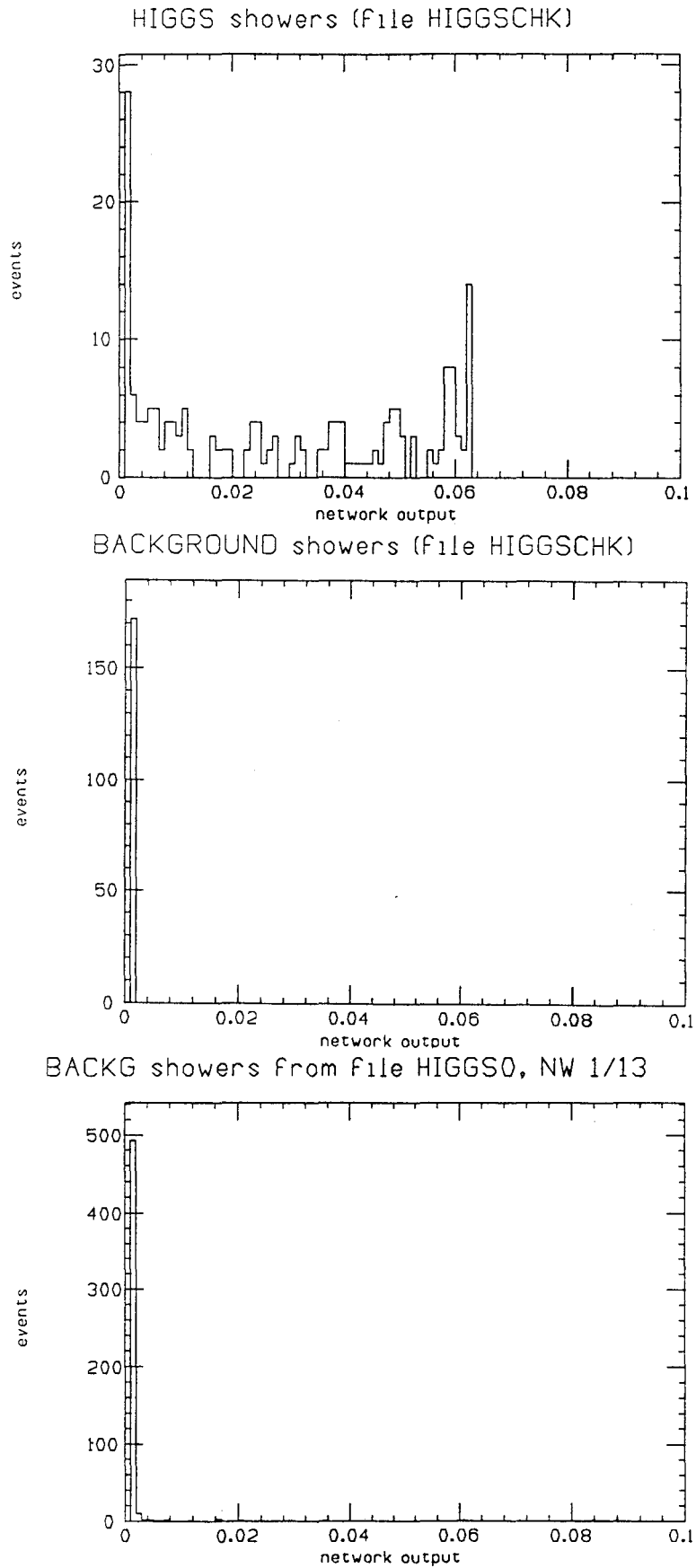
Fig. 10 Response of the trained network to showers from \text{Higgs} \rightarrow \gamma\gamma photons and to backgrounds. The network was trained with equal numbers of events containing Higgs showers and background events.
