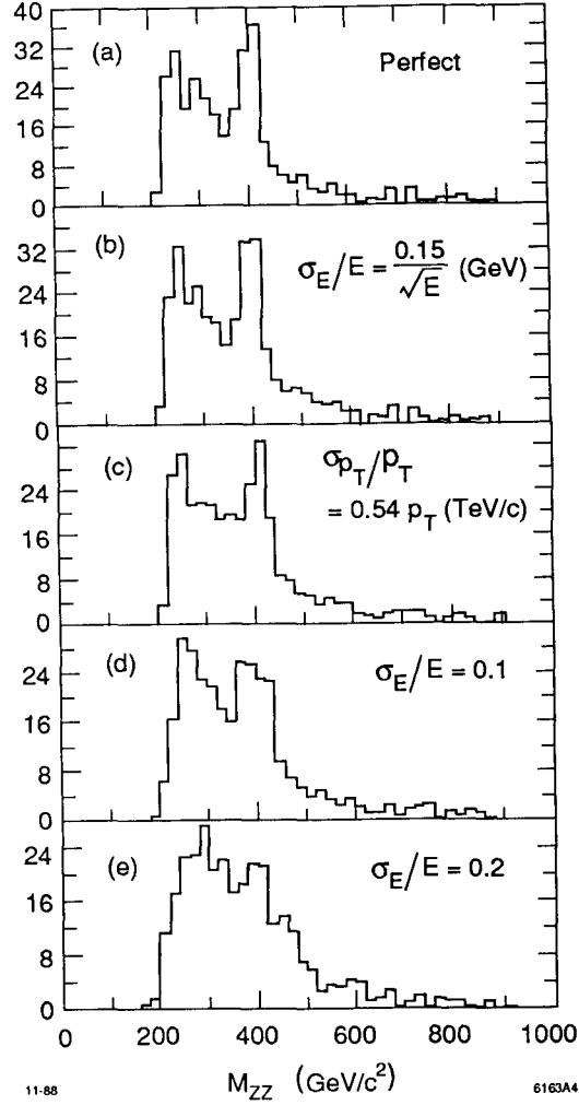
Fig. 8. Z -pair mass distributions for various energy or momentum resolutions for H \rightarrow ZZ \rightarrow 4\ell^\pm for a 400 \text{GeV}/c^2 Higgs boson, along with the background from continuum ZZ production.
