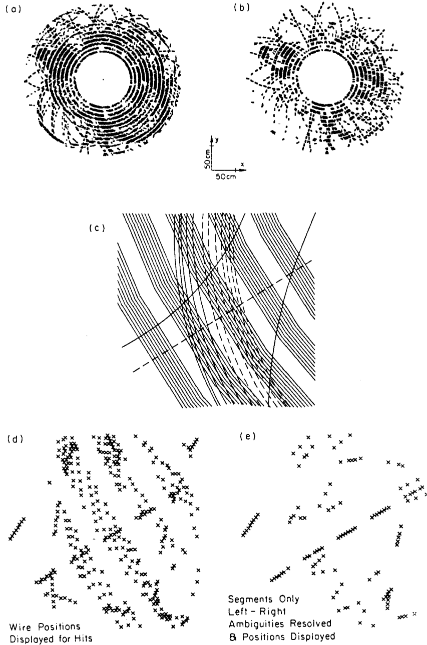
Fig. 12. (a) All of the digitizations for the Higgs event shown in Fig. 10, including those from minimum bias background events. (b) Digitizations for this event which are included in track segments, as defined in the text. (c) Tracks from the original event in an enlarged region in the outer five superlayers in the region around the muon at the lower right. (d) All of the digitizations in the event in the enlarged region of (c) (the digitizations are displayed at the locations of the hit wires). (e) Only those digitizations which form track segments in the enlarged region. Here, the left-right ambiguities have been resolved, the drift times have been converted to distances, and the digitizations are displayed at the positions of closest approach of the tracks to the wires.
