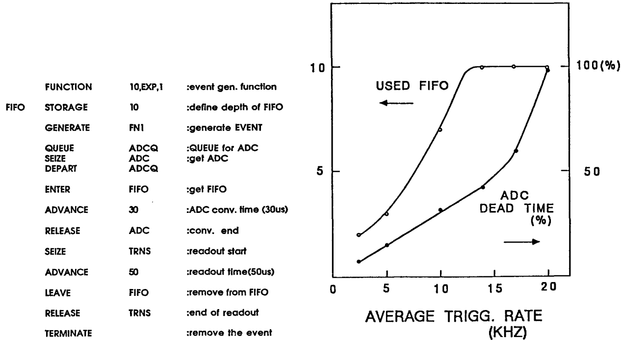
Fig. 4: List of GPSS program
