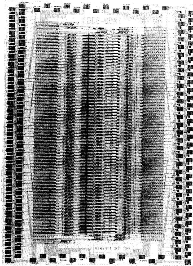
Fig. 2 Layout of the 64 channel preamp/shaper/discriminator chip.
