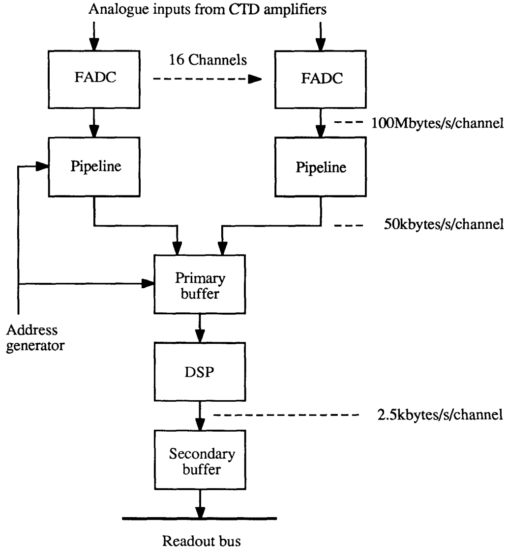
Fig 1. Front end data acquisition.
