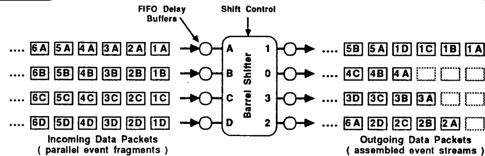
Figure 2 High Bandwidth Event Builder Using Simple TDM Switch
