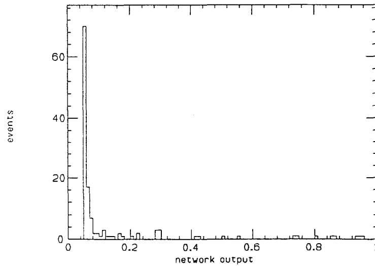
Fig. 11 Response of the trained network to showers from \text{Higgs} \rightarrow \gamma\gamma photons and to backgrounds. The network was trained with equal numbers of Higgs showers and background showers.
