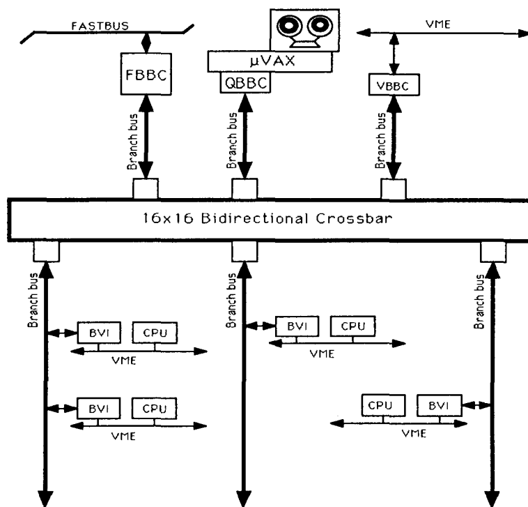
Figure 4. The bus switch used to interconnect data acquisition buses with VME processor farms.
