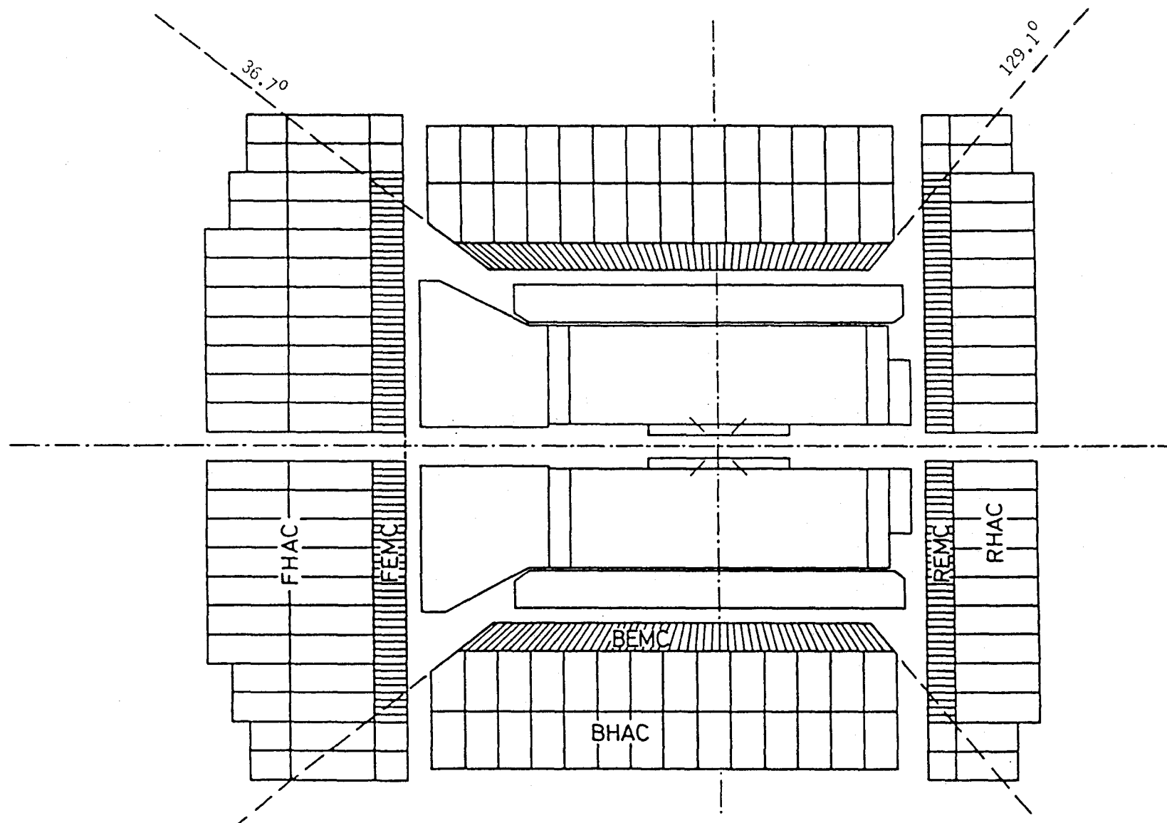
Figure 2. The Zeus High Resolution Calorimeter.
