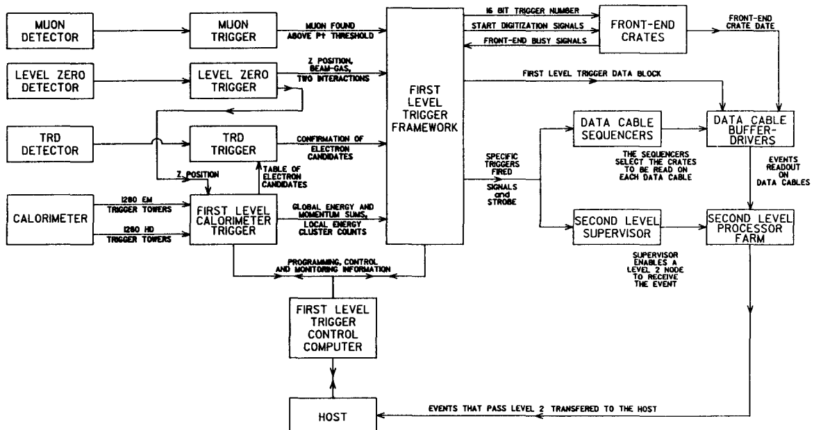
Figure 1. A block diagram of the D0 triggering and data acquisition system.
