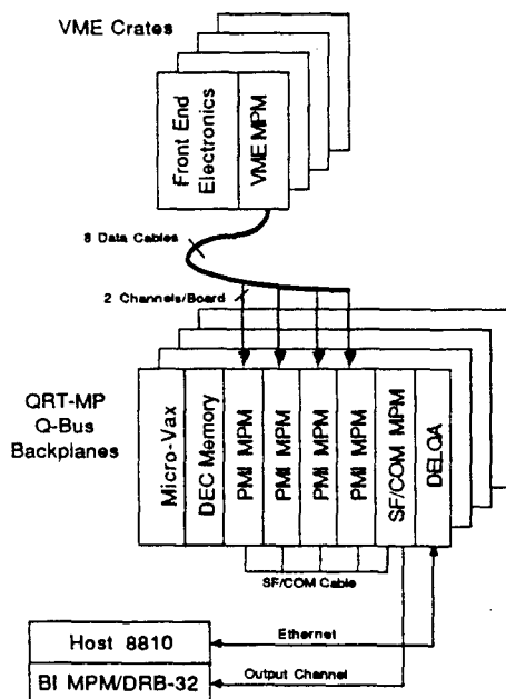
Fig. 2 Schematic of next generation D0 Level-2 node.
