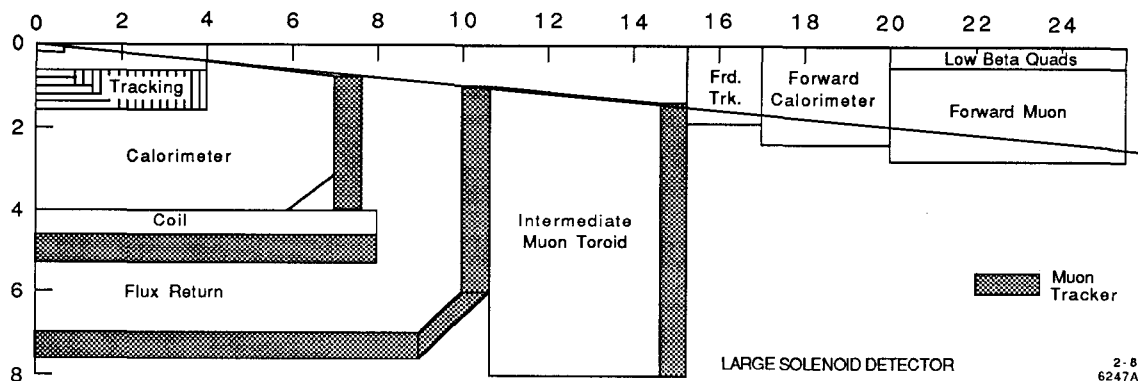
Fig. 4. Schematic view of the Large Solenoid Detector from the 1987 Berkeley Workshop. 10
