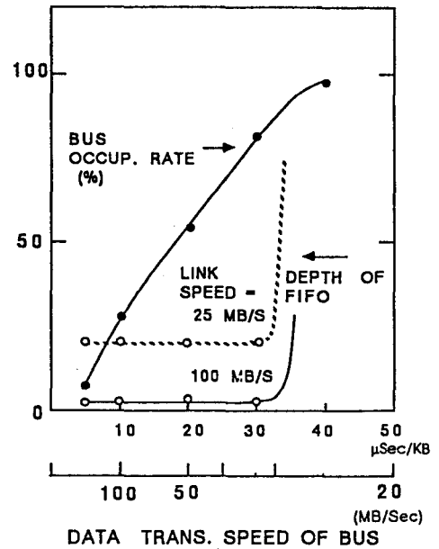
Fig. 10: Required depth of FIFO and the occupancy of BUS as a function the transfer speed of BUS
