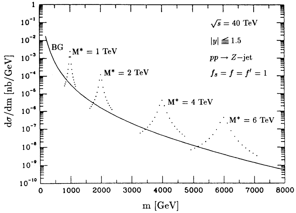
Fig. 1. The invariant mass distribution d\sigma/dm of excited quarks produced in pp collisions at the SSC versus invariant mass for various values of the excited quark mass, M^* . The solid curve represents the Z + jet background. Taken from Ref. 1.
