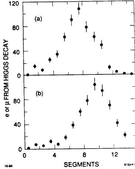
Fig. 13. (a) Distribution of the number of good segments out of 13 possible for the e 's and \mu 's from the Higgs decays. (b) Distribution of the number of total segments (good or OK) for the leptons from the Higgs decay.
