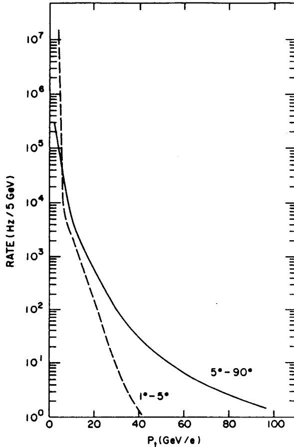
Fig. 3. The rate of particles (muons) exiting outer iron shielding in a typical detector versus the transverse momentum of the particle for two different angular regions. Taken from Ref. 6.
