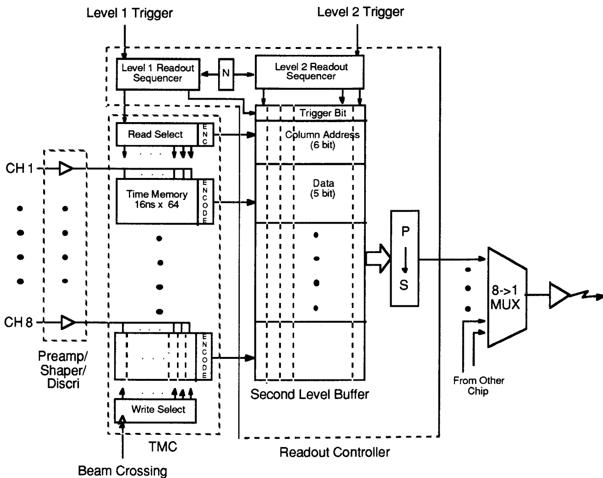
Fig. 8 Readout scheme of the time measurement system.
