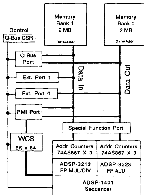
Fig. 3 Block diagram of multiport memory with floating point coprocessor.
