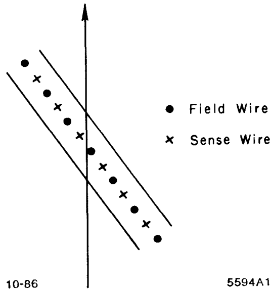
Fig. 2. Narrow tilted jet cell with radial track.
