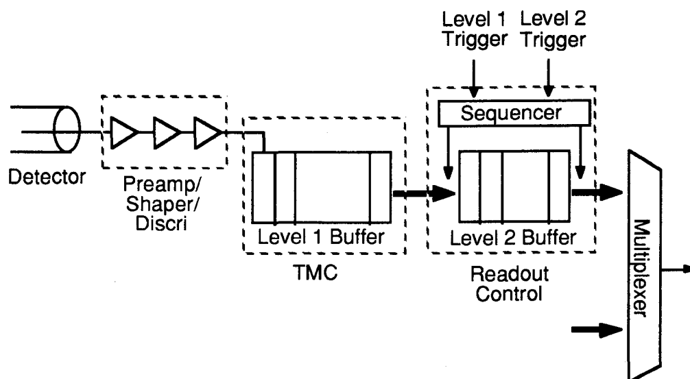
Fig. 1 A schematic diagram of the front-end electronics for time measurement system.
