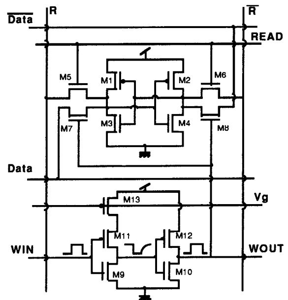
Fig. 4 Basic Cell of the TMC.
