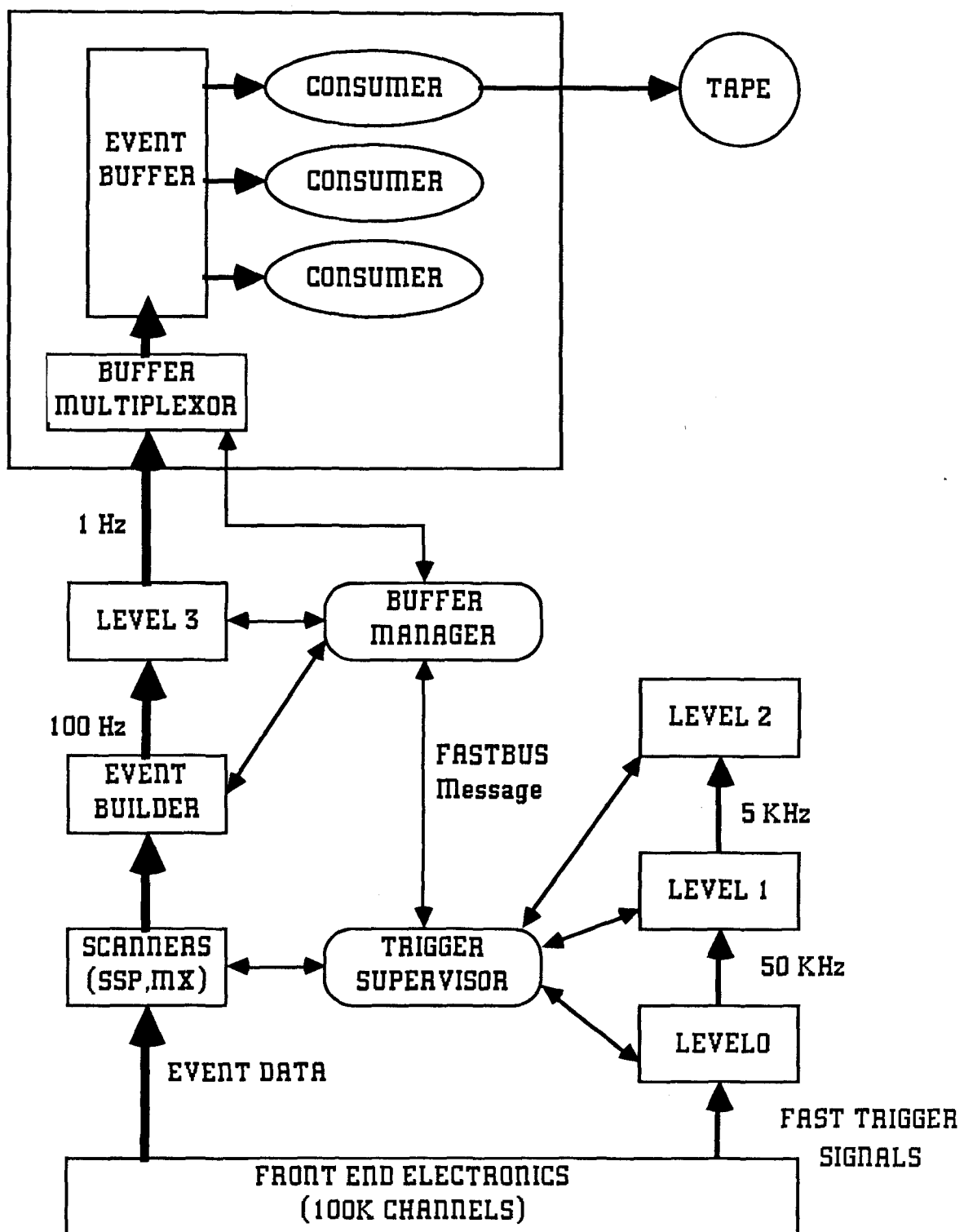
Fig. 3: DAQ PIPELINE
