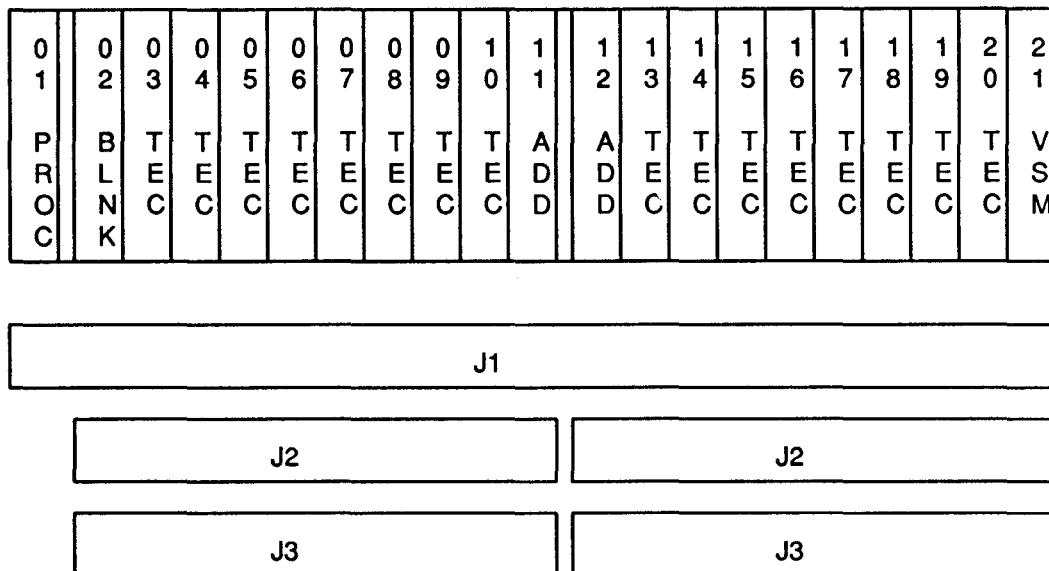
Figure 10. Assignment of modules to slots in trigger VME crates with backplane divisions shown below. Trigger Encoder cards are labelled TEC, Adder Cards are labelled ADD, the VME Service Module is labelled VSM, there is a blank slot labelled BLNK, and the Crate Processor Board is labelled PROC. The J1 bus is connected to all 21 slots. The J2 and J3 busses are broken between slots 11 and 12 and do not continue to slot 1. All user-defined lines on the continuous sections of the J2 and J3 busses are linked together.
