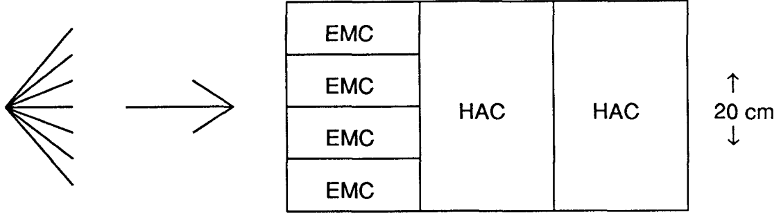
Figure 3. A particle from an interaction entering an ideal supertower.
