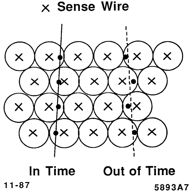
Fig. 3. Layers of straw tubes in a superlayer with every other layer staggered by the straw tube radius. A single in-time track will appear as a series of hits on the wires on alternate sides of the track. The left-right ambiguity is easily resolved locally. A track from an out-of-time bunch crossing will produce hits which are displaced from possible tracks by at least 16 ns in drift time.
