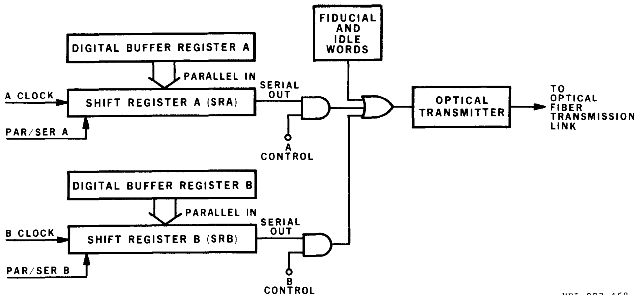
Fig. 4. Time division multiplexer.
