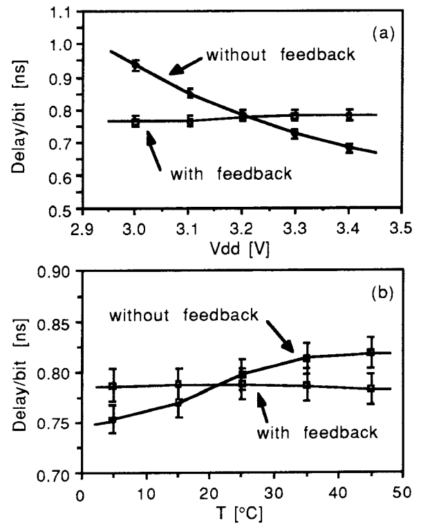
Fig. 7 (a) Supply voltage dependence of the delay element. (b) Temperature dependence of the delay element.
