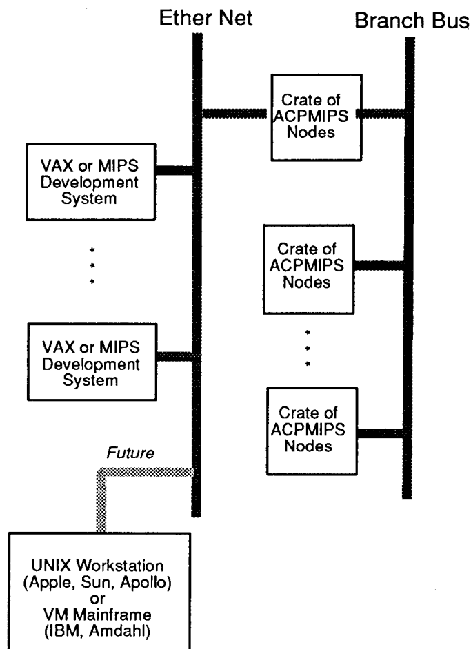
Figure 3. Second generation ACP multiprocessor systems allow any VMS or UNIX processor or workstation to take part.
