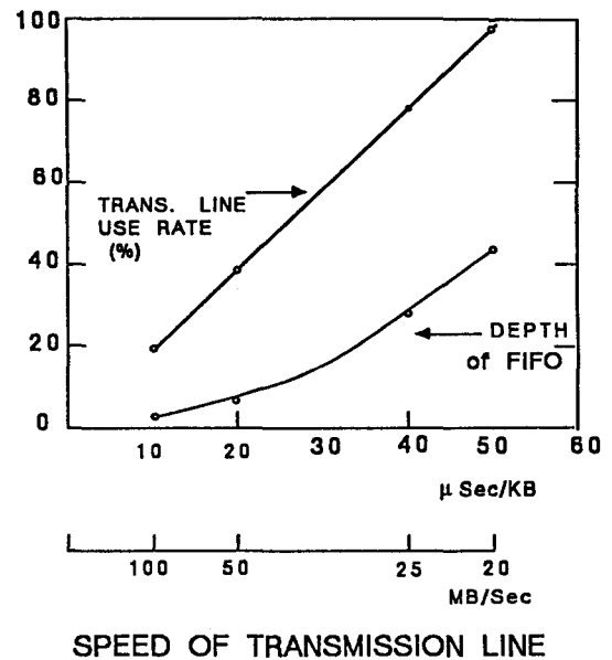
Fig. 8: Simulated results on the required FIFO depth and the use rate of the transmission line as a function of the speed
