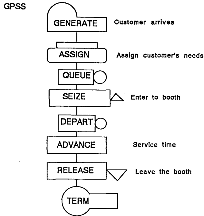
Fig. 1: A Block diagram of GPSS
