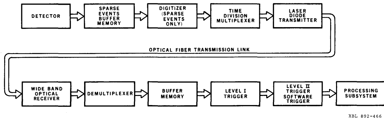
Fig. 3. Simplified block diagram for optical fiber transmission in SSC detector system where signals are multiplexed before the Level I Trigger.
