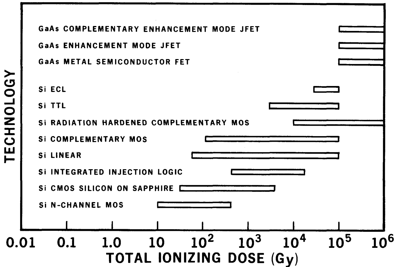
Fig. 14. Estimated ranges of total dose damage susceptibility for silicon and gallium arsenide devices.
