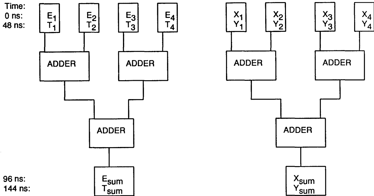
Figure 6. Half (either HAC or EMC part) of the adder tree network on each Trigger Encoder Card. E_i represents the total energy in the supertower section, T_i is E_i \sin \theta_i (transverse energy), X_i is E_i \sin \theta_i \cos \phi_i ( E_x ) and Y_i is E_i \sin \theta_i \sin \phi_i ( E_y ). The elapsed time is shown on the left.
