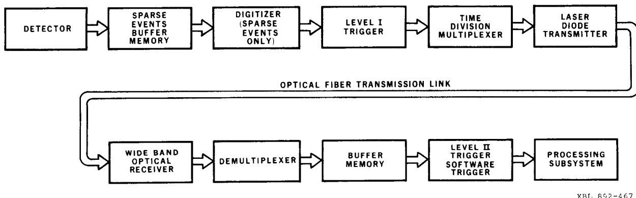
Fig. 2. Simplified block diagram for optical fiber transmission link in SSC detector system where signals are multiplexed after the Level I Trigger.
