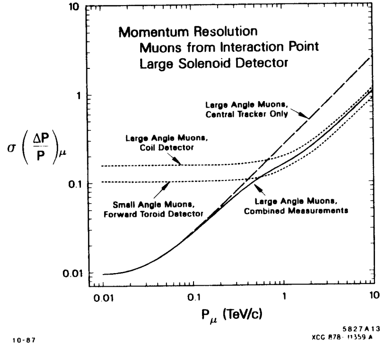
Fig. 6. Momentum resolution for measurement of large-angle and small-angle muons in the Large Solenoid Detector (from Ref. 10).
