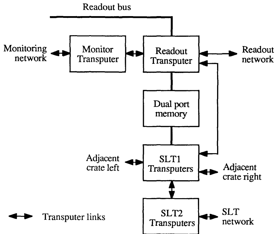
Fig 2. Crate readout
