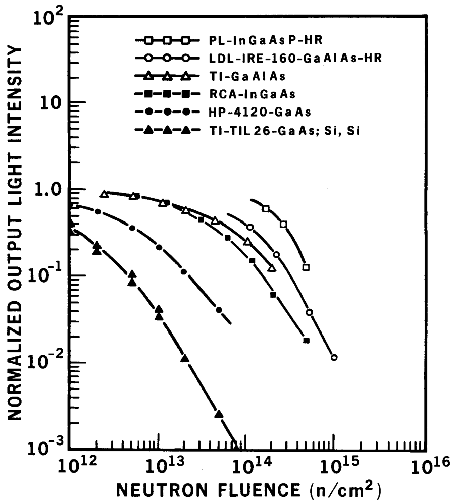
Fig. 6. Normalized light output as a function of the neutron fluence for various LEDs under constant current operating conditions.
