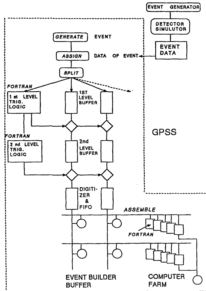
Fig. 2: Schematic diagram of a data acquisition system in GPSS
