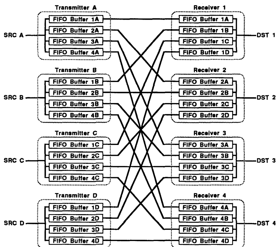
Figure 3 "Logical" Switch Operation
