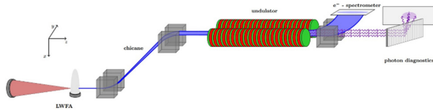
Figure 1: Schematic layout of a LWFA-based scTGU radiation source [2].
