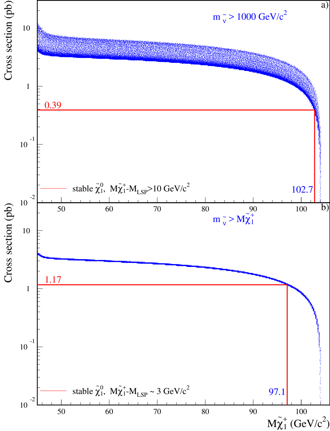
Figure 28: Expected cross-sections in pb at 208 GeV (dots) versus the chargino mass in a) for \Delta M > 10 GeV/c 2 and b) for \Delta M \sim 3 GeV/c 2 . The spread in the dots originates from the random scan over the parameters \mu and M_2 . A heavy sneutrino ( m_{\tilde{\nu}} > 1000 GeV/c 2 ) has been assumed in a) and m_{\tilde{\nu}} > M_{\tilde{\chi}_1^\pm} in b). The minimal cross-sections below the mass limits are indicated by the horizontal lines.
