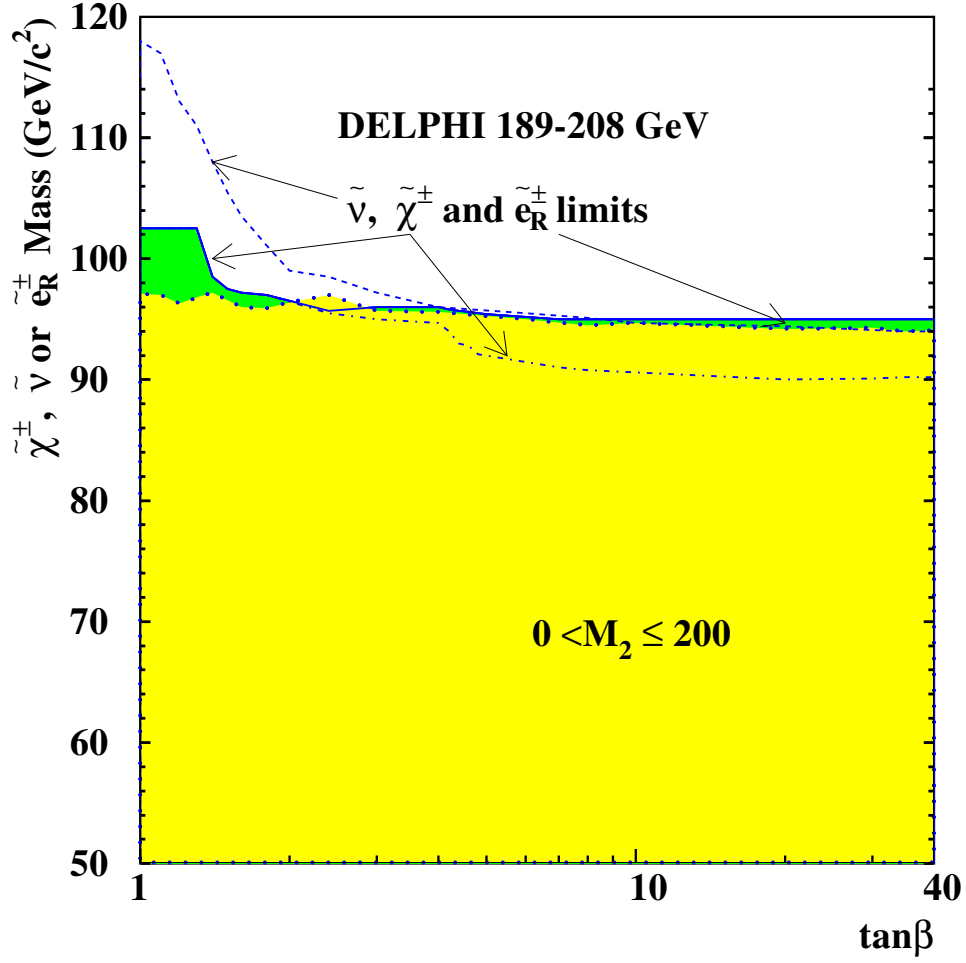
Figure 42: The minimum sneutrino mass (dark shading and the dashed curve) allowed by the slepton and neutralino searches, as a function of \tan \beta , together with the limits on the chargino mass (solid curve and dash-dotted curve), and the \tilde{e}_R mass (dotted curve and the light shading). The chargino mass limit indicated by the solid curve and the sneutrino and selectron mass limits were obtained assuming no mass splitting in the third sfermion family ( A_\tau - \mu \tan \beta = 0 in particular). The selectron mass limit is valid for M_{\tilde{e}_R} - M_{\tilde{\chi}_1^0} > 10 \text{GeV}/c^2 . The chargino mass limit indicated with the dash-dotted curve was obtained allowing for mass splitting in the third sfermion family, with A_\tau = A_b = A_t = 0 .
