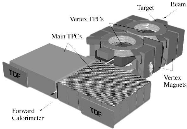
Fig. 2. The NA49 experimental setup.
