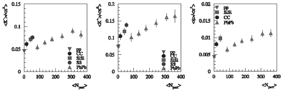
Fig. 10. The meson/pion ratio for kaons (both charges) and \Phi as a function of the number of participants for different colliding systems.
