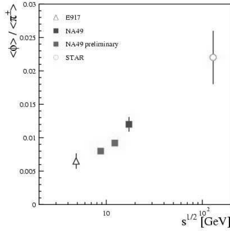
Fig. 9. The average \Phi meson multiplicity, normalised to pions, as a function of energy.
