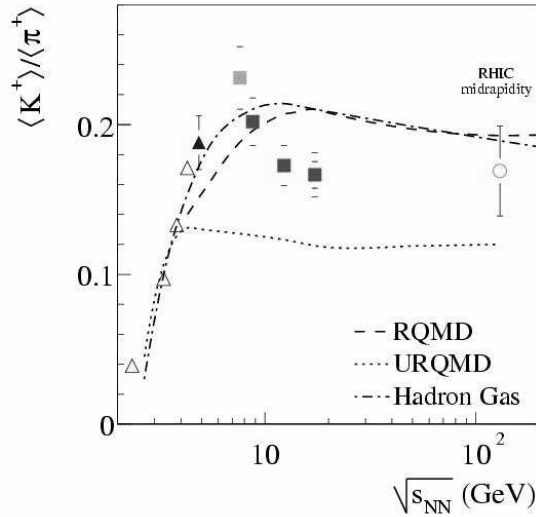
Fig. 5. Same data as in Fig. 4, together with a RHIC point, and the new 20 GeV/ c point. The curves correspond to various model descriptions.
