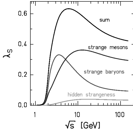
Fig. 6. The Wroblewski strangeness suppression factor \lambda as a function of energy, calculated in the model of Redlich et al. [7].
