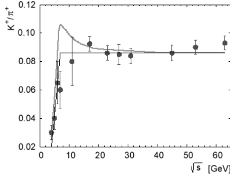
Fig. 8. Midrapidity K^+/\pi^+ ratio evolution with energy. Data from p - p (points) are interpolated by a straight line, and the resulting ratio for Pb-Pb collisions is shown by the thick line.
