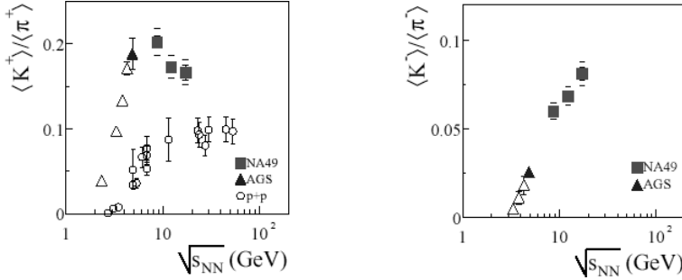
Fig. 4. The K^+/\pi^+ and K^-/\pi^- ratios for central Pb–Pb collisions, together with p – p data points.
