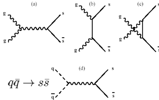
Fig. 1. Main diagrams contributing to strangeness production.
