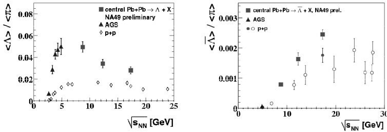
Fig. 12. \Lambda and \bar{\Lambda} multiplicities, normalised to pions, as a function of energy for central nuclear collisions.
