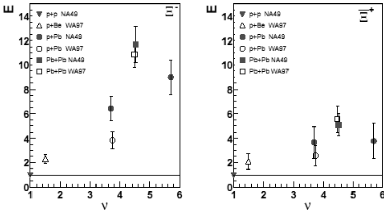
Fig. 14. Enhancement of hyperon production in nucleus–nucleus and proton–nucleus collisions, as a function of the number of collisions \nu .
