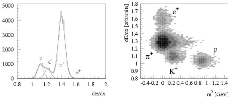
Fig. 3. Particle identification via ionisation energy loss and time of flight measurement in the NA49 experiment.
