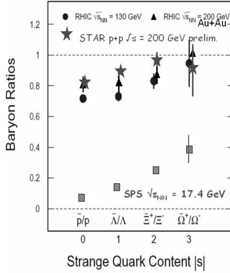
Fig. 16. \bar{B}/B ratios for elementary and nuclear collisions at RHIC and SPS, as a function of the strangeness content
