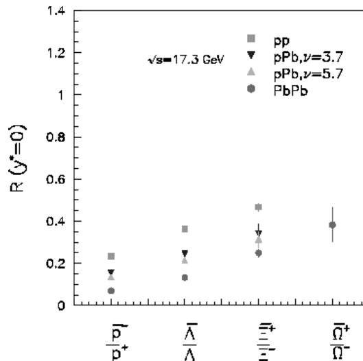
Fig. 15. \bar{B}/B ratio at midrapidity for elementary, hadron–nucleus and nucleus collisions at 158 GeV/ c .
