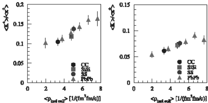
Fig. 11. Same ratios as in Fig. 10, as a function of mean collision density.
