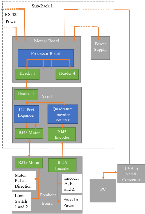
Figure 2: Architecture of the 64-axis motion controller.
