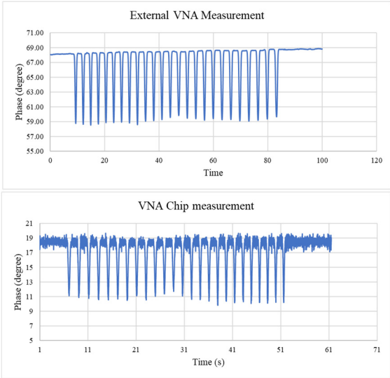
Figure 5: Phase vs time measured during beadpull using (Upper) external VNA and (Lower) VNA chip inside the bead-pull control system.
