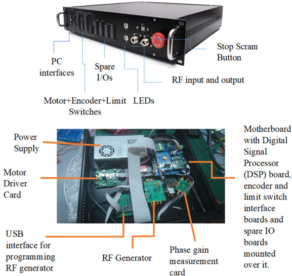
Figure 4: Major components of the bead-pull control system.
