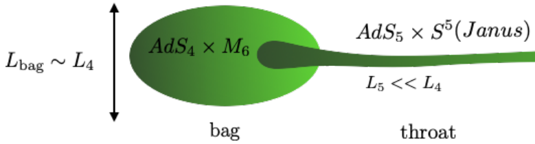
Figure 3.1: The manifold described in the text, is comprised by one (or two at most) semi-infinite AdS_5 \times S^5 or Janus throat of radius L_5 attached on a compact ‘bag’ of typical size L_{\text{bag}} \sim L_4 \gg L_5 .
