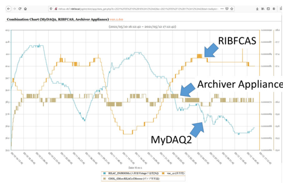
Figure 2: Example of accessing data using Firefox and displaying Archiver Appliance, MyDAQ2, and RIBFCAS archived data on jqPlot-based chart at the same time.
