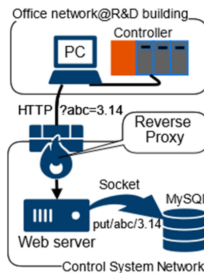
Figure 3: System chart of sending archiving data from the R&D building to MyDAQ2 through a reverse proxy.
