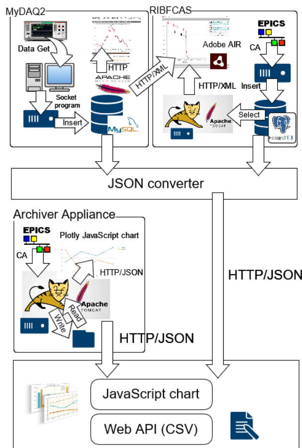
Figure 1: System chart of linkage methods with existing systems. The clients obtain the archived data through the JavaScript chart or Web API.
