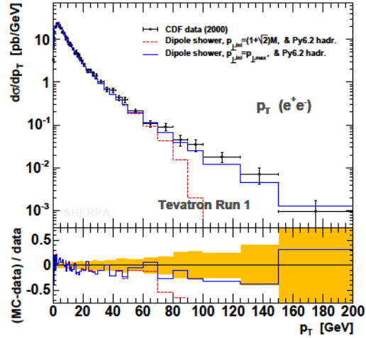
Figure 2: The p_{\perp} distribution of the Z boson in Drell-Yan processes at the Tevatron. The new dipole shower is confronted with data from [31].
