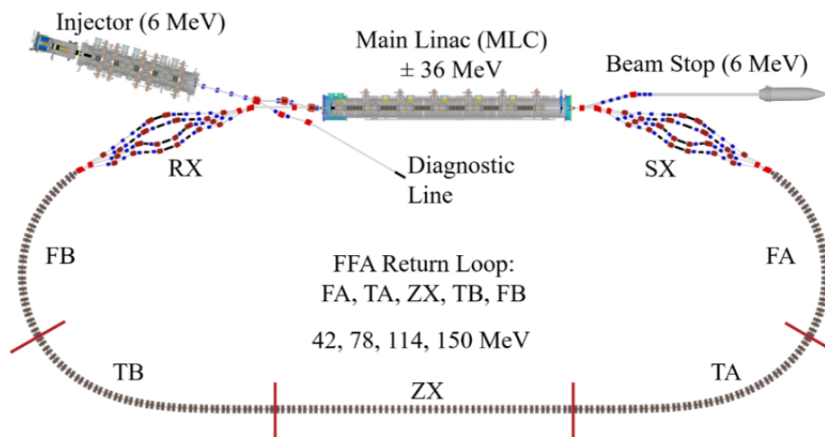
Figure 1: The four-turn configuration of CBETA.
