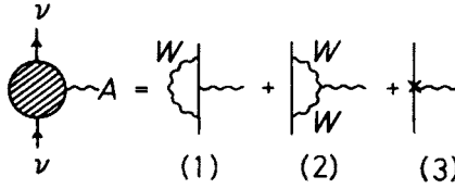
Fig. 3.7. The \nu\nu A vertex diagrams
