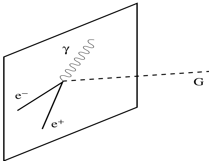
Figure 2. The confinement of matter to the brane, while gravity propagates in the bulk (from [3]).
