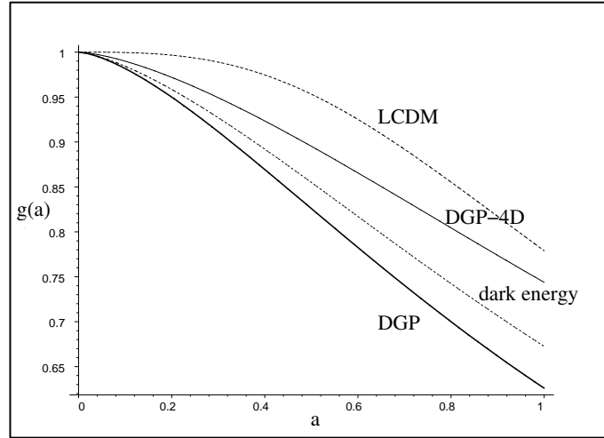
Figure 5. The growth factor g(a) = \Delta(a)/a for LCDM (long dashed) and DGP (solid, thick), as well as for a dark energy model with the same expansion history as DGP (short dashed). DGP-4D (solid, thin) shows the incorrect result in which the 5D effects are set to zero. (From [13].)
