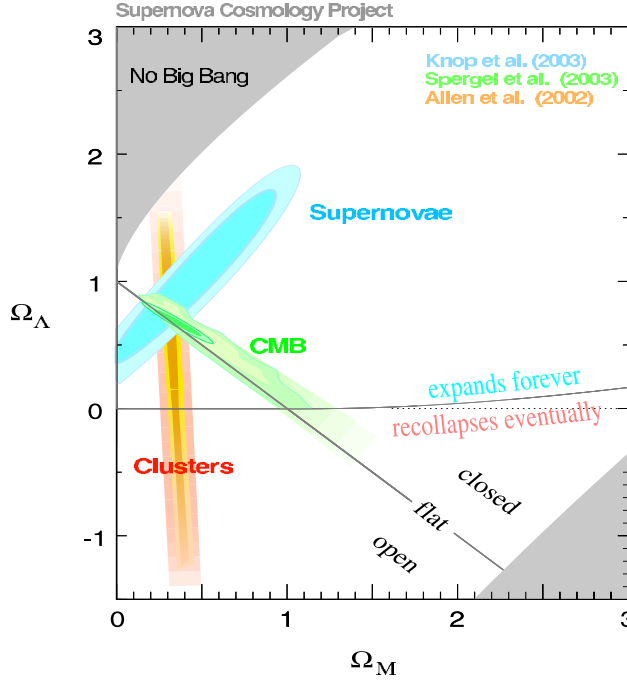
Figure 1. Observational constraints in the (\Omega_\Lambda, \Omega_M) plane (from [2]).
