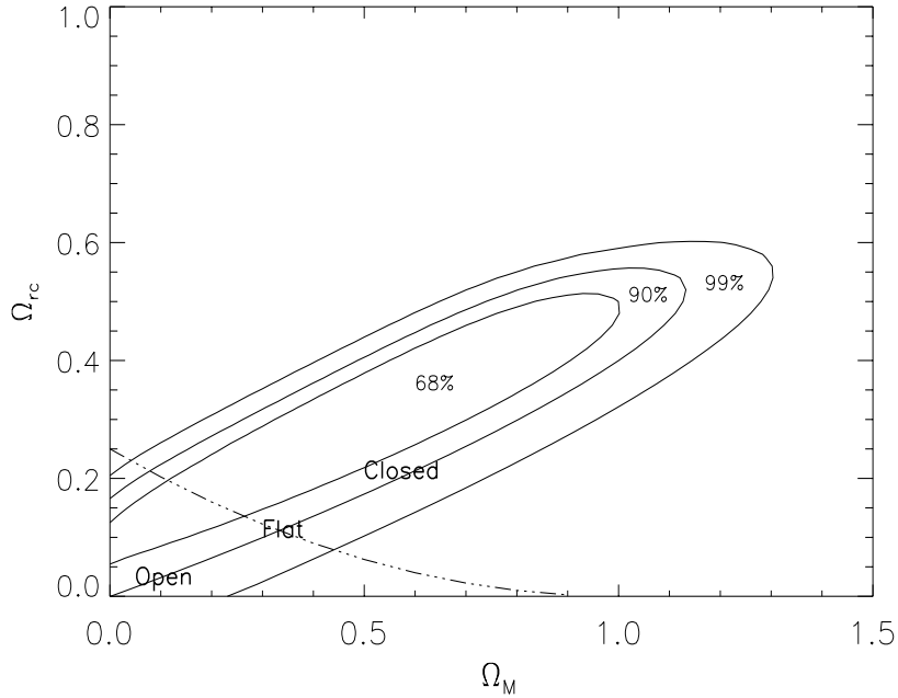
Figure 4. Constraints from SNe redshifts on DGP models, where \Omega_{r_c} = (2H_0 r_c)^{-2} . (From [12].)
