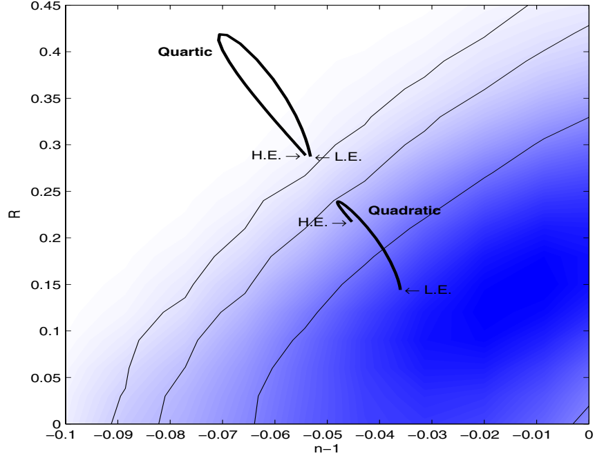
Figure 3. Constraints from CMB and large-scale structure data on inflation models with quadratic and quartic potentials, where R is the ratio of tensor to scalar amplitudes and n is the scalar spectral index. The high energy (H.E.) and low energy (L.E.) limits are shown, with intermediate energies in between, and the 1-, 2- and 3- \sigma contours are also shown. (From [8].)
