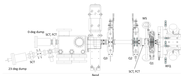
Figure 3: Schematic drawing of the test bench.
