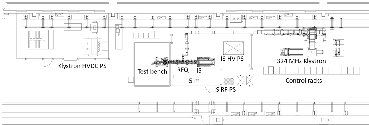
Figure 1: Schematic layout of the 3 MeV linac.
