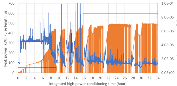
Figure 4: Conditioning history of the new RFQ. The orange line shows the stored peak power (absolute value is not calibrated), the black line represents the pulse width, and the blue line indicates the vacuum pressure.
