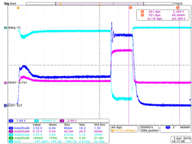
Figure 5: Typical beam pulse. Blue: RFQ input. Magenta: RFQ exit. Cyan: 0 deg beam dump.
