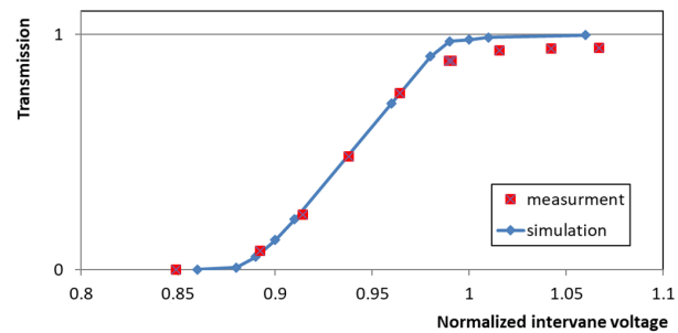
Figure 6: Measured and simulated transmission of the RFQ. The red squares and blue diamonds are measured and simulated transmission of the RFQ, respectively.
