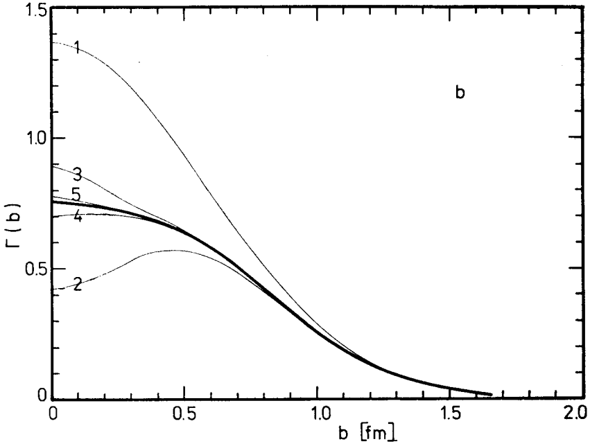
Fig. 3. a) Differential cross section \frac{d\sigma}{dt} and b) impact parameter profile \Gamma(\vec{b}) calculated to the first (1), second (2), third (3), fourth (4), fifth (5) and ninth order of the multiple scattering expansion for the Gaussian density function (3.4) and Gaussian quark amplitudes (3.2) with the typical values of parameters
