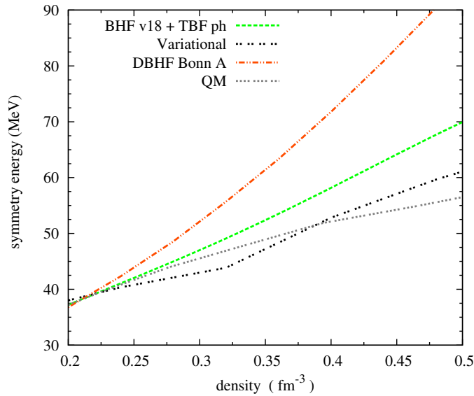
Figure 10. The symmetry energy above saturation density calculated with the different EoS included in Fig. 9, with exception of the EoS from the chiral approach. Figure taken from Ref. [27].
