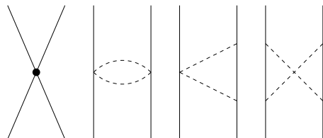
Figure 3. Chiral two-body forces. The full lines indicate nucleon propagation, the dashed lines indicate pion propagation, which results in a finite range interaction. A simple crossing between two nucleon lines indicates a point interaction, and a full dot correspond to a derivative coupling.
