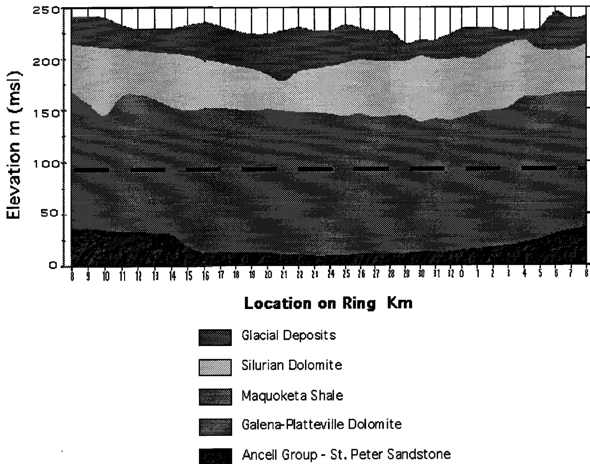
Figure 2 Geology of Booster region The dotted line indicates the Booster tunnel elevation
