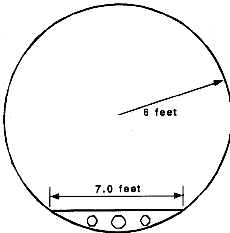
Figure 3 Tunnel cross section
