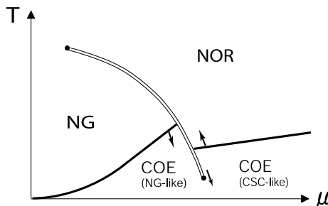
Fig.1. Schematic phase diagram with two light (up and down) quarks and a medium heavy (strange) quark. The arrows show how the critical point and the phase boundaries move as the strange-quark mass increases.
