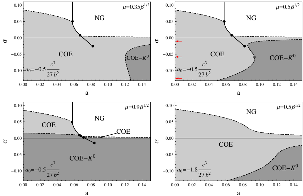
Fig. 2. Ginzburg–Landau phase diagrams with strange quark mass and kaon condensation.
