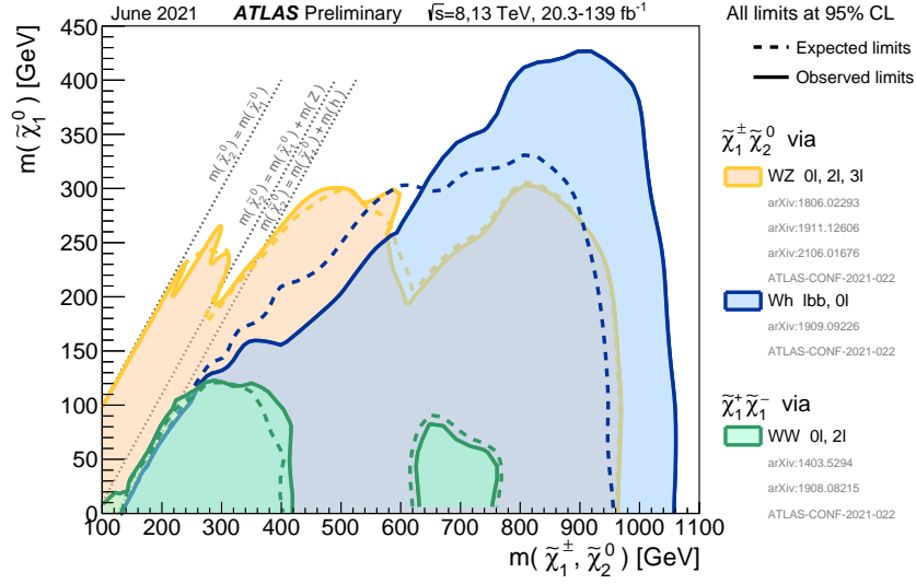
Figure 12: The 95% CL exclusion limits on \tilde{\chi}_1^\pm \tilde{\chi}_1^- and \tilde{\chi}_1^\pm \tilde{\chi}_2^0 production with SM-boson-mediated decays, as a function of the \tilde{\chi}_1^\pm , \tilde{\chi}_2^0 and \tilde{\chi}_1^0 masses. The production cross-section is for pure wino \tilde{\chi}_1^\pm \tilde{\chi}_1^- and \tilde{\chi}_1^\pm \tilde{\chi}_2^0 . Each individual exclusion contour represents a union of the excluded regions of one or more analyses.
