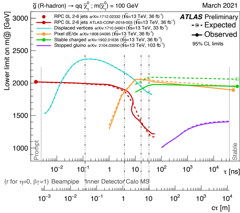
Figure 19: Constraints on the gluino mass-vs-lifetime plane for a split-supersymmetry model with the gluino R-hadron decaying into a gluon or light quarks and a neutralino with mass of 100 GeV. The solid lines indicate the observed limits, while the dashed lines indicate the expected limits. The area below the curves is excluded. For the displaced vertices result the expected and observed limits are identical. For the stopped gluino result the limit extends to larger lifetimes (not quoted here, see reference). The analyses have sensitivity at lifetimes other than those shown, but only the limits at tested lifetimes are shown. The dots represent results for which the particle is assumed to be prompt or stable. In this context, stable means escaping the detector.
