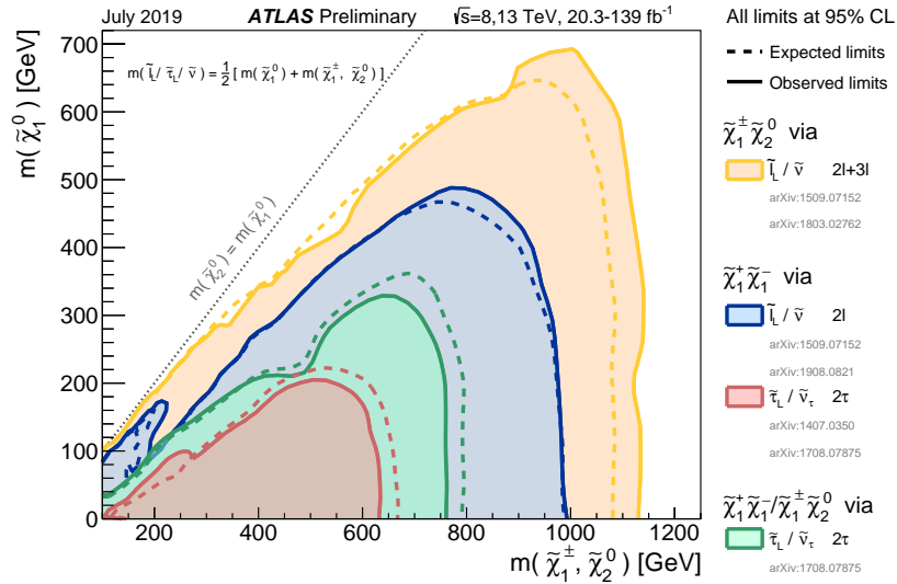
Figure 11: The 95% CL exclusion limits on \tilde{\chi}_1^+ \tilde{\chi}_1^- and \tilde{\chi}_1^+ \tilde{\chi}_2^0 production with \tilde{\ell} -mediated decays, as a function of the \tilde{\chi}_1^+ , \tilde{\chi}_2^0 and \tilde{\chi}_1^0 masses. The production cross-section is for pure wino \tilde{\chi}_1^+ \tilde{\chi}_1^- and \tilde{\chi}_1^+ \tilde{\chi}_2^0 . Each individual exclusion contour represents a union of the excluded regions of one or more analyses.
