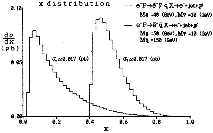
Fig. 3. x distribution d\sigma/dx for (1.1) e^-p \rightarrow e^-q\bar{q}X and (1.2) e^-p \rightarrow e^-q\bar{q}qX . Parameters are M_{\tilde{e}} = 50 GeV and M_{\tilde{q}} = 150 GeV for (1.1) and M_{\tilde{\gamma}} = 10 GeV and M_{\tilde{e}} = 40 GeV for (1.2). SUSY parameters are \mu = 100 GeV and \tan \theta_\nu = 1
