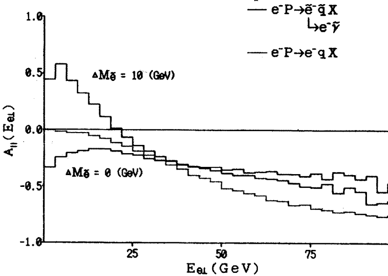
Fig. 4. Differential left-right asymmetry A_{||}(E_{eL}) for e^-p \rightarrow e^-q\bar{q}X . Averaged selectron mass M_{\tilde{e}} = 40 GeV is commonly adopted. Dotted line is for the background process e^-p \rightarrow eq\bar{q}X
