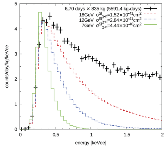
Fig.1. Observed scaled energy spectrum compared with that of simulation with 7 GeV, 12 GeV, and 18 GeV WIMP masses.
