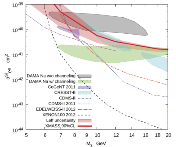
Fig.2. Upper limit at 90% C.L. on spin independent elastic WIMP cross section compared with other experiments.
