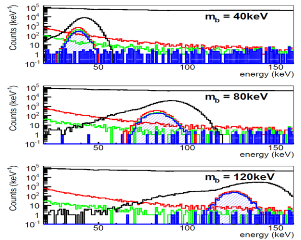
Fig. 7. Scaled energy distributions. Data shows continuous distributions in each reduction step with optimized cut for 40, 80, 120 keV vector boson masses. Distributions with bump show signal simulations.
