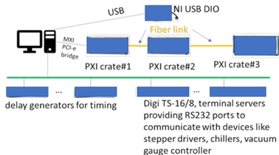
Figure 2: Hardware directly connected to control PC.
