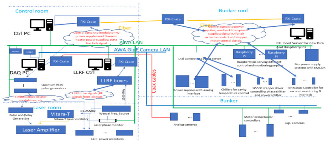
Figure 1: AWA control and DA system topology.
