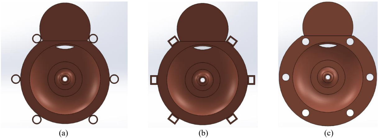
Figure 1: Cooling System Designs. a) Tangential Pipe. b) Tangential Duct. c) Internal Pipe.
