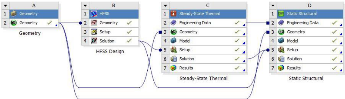
Figure 2: RF-Thermal-Structural-RF Coupling analysis in Ansys Workbench.
