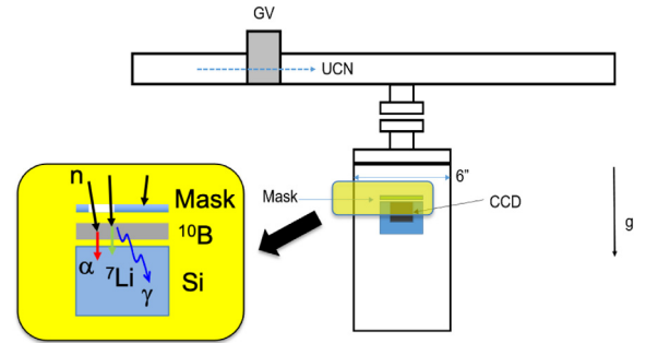
Fig. 2. The schematic of the experimental setup. The UCN flux to the detector chamber is controlled by a gate valve (GV). The CCD detector faces up. Experiments are conducted both with and without a mask on the top of the CCD back side. The readout electronics (outside the vacuum chamber), the vacuum interface for the bCCD data cables, and on-board electronics (inside the vacuum chamber) are not shown.
