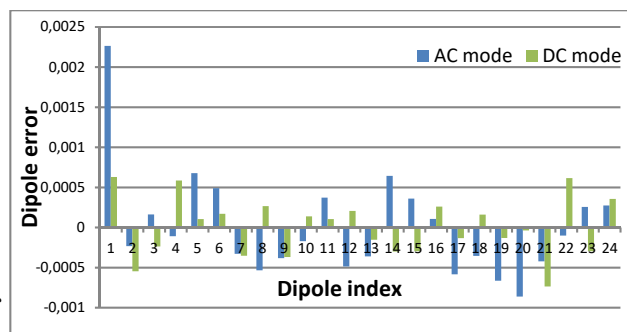
Figure 3: The DC and AC dipoles field error.
