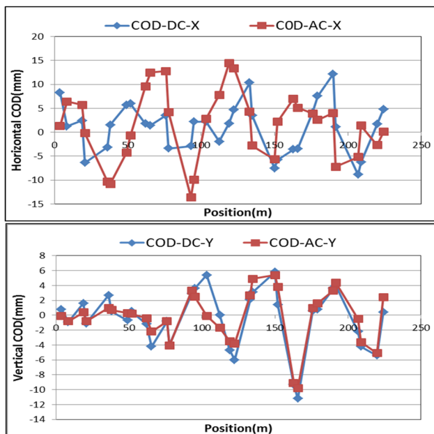
Figure 2: Bare orbits for DC mode and AC mode.
