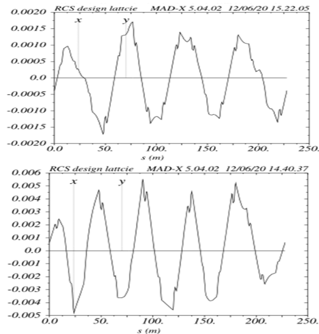
Figure 4: Horizontal closed orbit distortion from dipole field errors (The top is DC mode, the below is AC mode).
