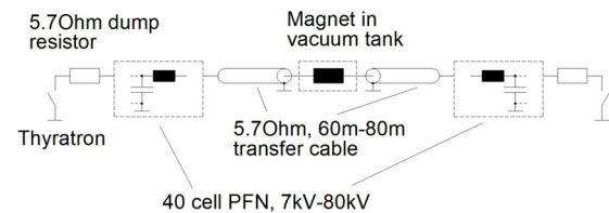
Figure 2: EE-Kicker schematic diagram.
