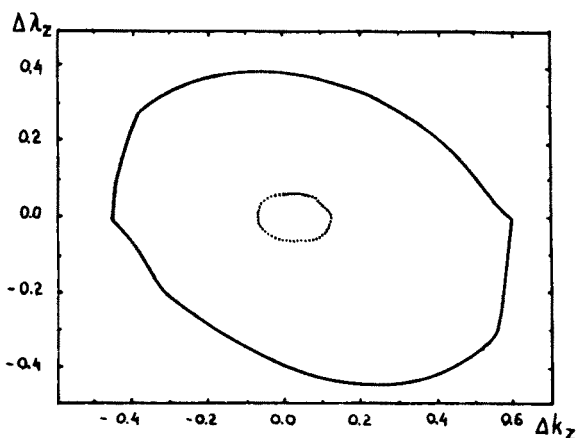
Fig. 7. The bounds on the \Delta k_z and the \Delta \lambda_z following from measurements of the \sigma_{T(e^-e^+ \rightarrow W^-W^+)} fulfilled with a precision of about 5% at energies up to 200 (solid line) and 500 GeV (dotted line).
