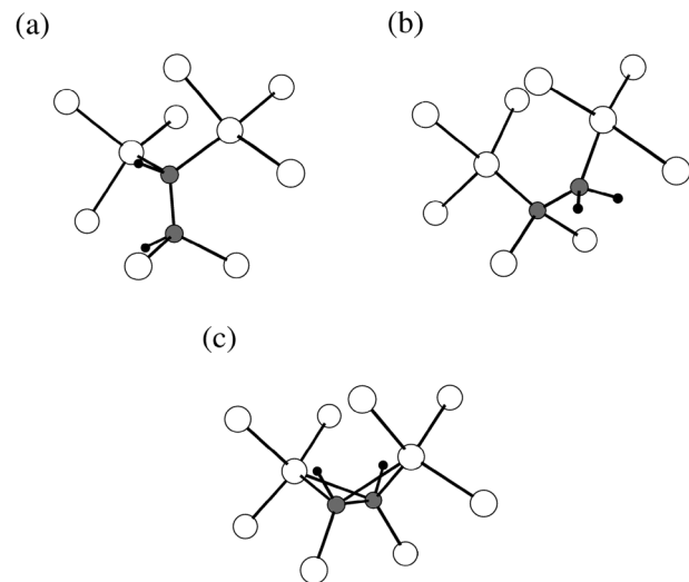
FIG. 2. Schematic of the three possible structures of the C_2H_2 split-interstitial defect: (a) The (C_2H_2)_{\langle 100 \rangle} , (b) the (C_2H_2)_{BC} , and (c) the (C_2H_2)_{\langle 110 \rangle} configuration. Reproduced with permission from Leary et al. , Phys. Rev. B 57 , 3887–3899 (1998). Copyright 1998 American Physical Society.
