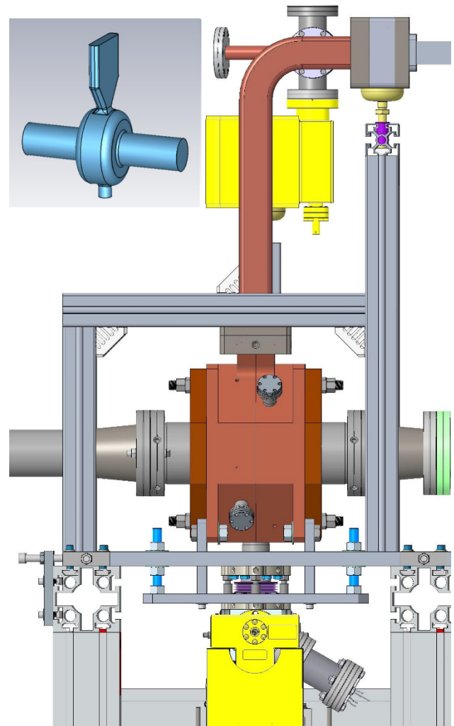
Figure 1: Vacuum model of the 1.4 GHz warm cavity. The L shape rectangular waveguide on the top is the FPC, with RF window on the top right, and an arc detector port with line of sight on the left of the window. The tuner is on the bottom. There are four ports on the cavity wall, with two shown in the plot and the other two on the back side, that serve as ports for fixed tuners and pickup couplers. The figure on the top left is the vacuum model of this cavity.
