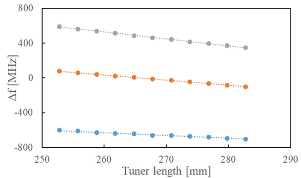
Figure 2: Three resonances (showed as three lines in the plot) in the tuner that are adjacent to 1.4 GHz, with x axis the tuner length and y axis the frequency away from 1.4 GHz.
