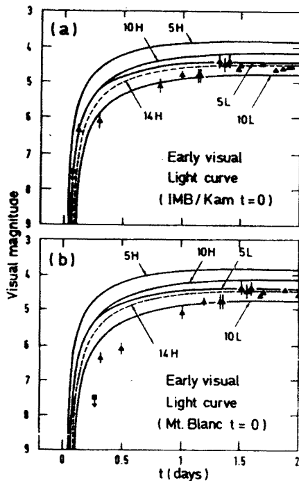
Fig. 8. SN1987A light curve during the first few days. (Woosley 1988) compared to various theoretical calculations using an exagerately large range of parameters, and assuming that either the IMB/Kamioka/Baksan detections trace the time of collapse (a), or that the Mt Blanc observation is at the time of collapse (b). Only the former is seen to provide consistency between the optical and neutrino timing, despite the short delay (2 hours) this implies
