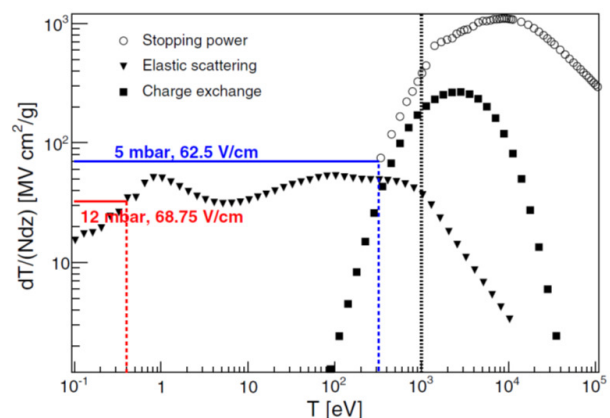
Figure 1: The mass stopping power of \mu^+ in He gas. The vertical blue and red dashed lines show the resulting equilibrium energies at two experimental conditions, respectively [7].
