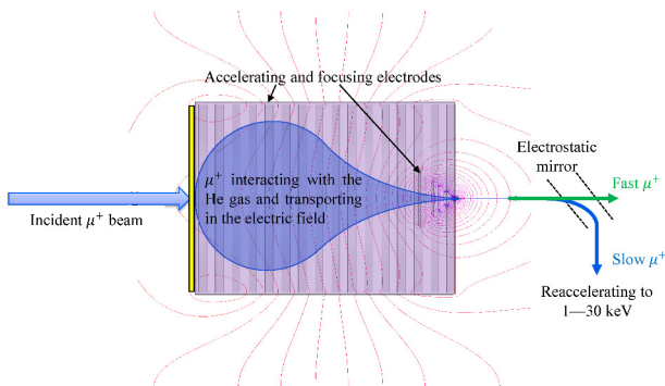
Figure 2: Preliminary scheme for frictional cooling of \mu^+ .
