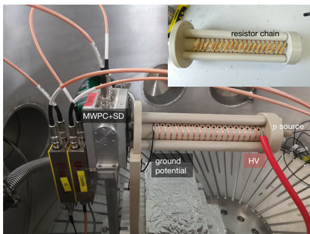
Figure 5: The experimental setup for the HV stability test of the accelerating grid. The inset shows the resistor chain welded to the accelerating grid. The Silicon Detector (SD) together with the MultiWire Proportional Chamber (MWPC) was used for the proton energy measurement. However, due to a low signal-to-noise ratio, there was a large uncertainty in the proton energy measurement. This would be greatly improved by using the SDD in future experiments.
