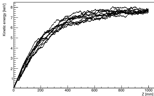
Figure 4: The kinetic energy of protons as a function of the drift distance in the longitudinal direction with an electric field of 336 V/cm in the He gas at a pressure of 5 mbar.
