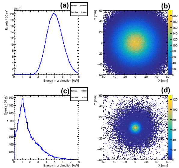
Figure 3: (a) The energy distribution and (b) the beam spot of the \mu^+ beam at the entrance of the gas cell. (c) The energy distribution and (d) the beam spot at the exit of the gas cell.
