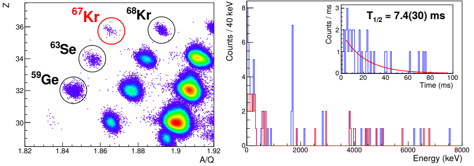
Fig. 1. Left: BigRIPS identification matrix of the fragments. Right: spectra of 67 Kr decays correlated with implantation events. The grey/red distribution shows events with a β particle detected in coincidence (βp emission). The black/blue one is obtained without this condition. The prominent peak at 1690(17) keV is assigned to the 2p decay. The inset shows the time spectrum of the decay events and the exponential fit.
