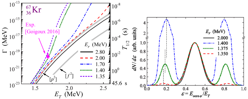
Fig. 2. IDDM calculations of ^{67}\text{Kr} for various resonance energies E_r in the ^{66}\text{Br}+p system. Left: correlation between 2p -decay width and Q_{2p} value ( E_T ), compared with the experimental value reported in these proceedings. The grey curves are three-body model calculations for pure p^2 and f^2 configurations. Right: energy sharing distribution between the two protons. The vertical dashed lines are the centroids of the peaks. Taken from [13].
