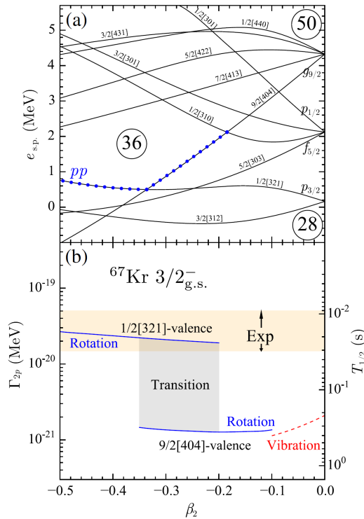
Fig. 3. Top: Nilsson levels ( \Omega[Nn_zA] ) of deformed core+ p potential as a function of the parameter \beta_2 . The dotted line is the occupied valence level. Bottom: 2p -decay width of ^{67}\text{Kr} as a function of \beta_2 . The solid and dashed lines are obtained with rotational and vibrational couplings respectively. Taken from [16].
