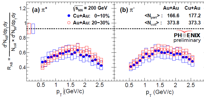
Figure 10. Pion nuclear modification factor, R_{AB} , in Cu+Au collisions at 200 GeV (closed circles) compared to that from Au+Au (open circles) at an equivalent N_{\text{coll}} . The results for \pi^+ are in panel a), for \pi^- in panel b).
