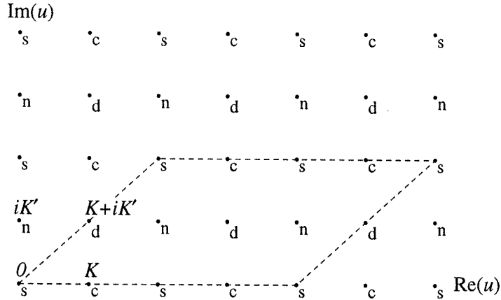
FIGURE A.4. A lattice of points for defining the Jacobian elliptic functions. The dashed outline shows a PP for the function sd\ u .
