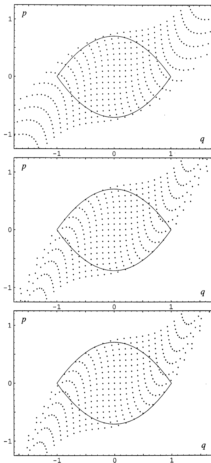
FIGURE 17.3. These graphics show for the anharmonic oscillator the results of applying once to the initial conditions shown in Figure 17.1 the non-linear part of the truncated Taylor maps \mathcal{T}_4 (top), \mathcal{T}_8 (middle), and \mathcal{T}_{12} (bottom) for time \tau = 1 .
