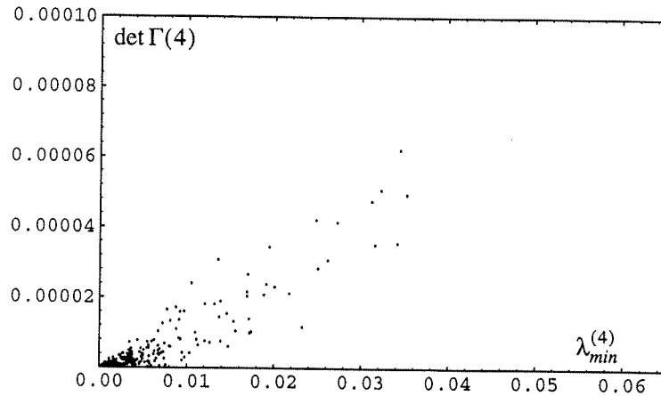
FIGURE 16.1. This plot shows the Gram determinant \det \Gamma(4) versus the minimum Gram eigenvalue \lambda_{\min}^{(4)} for 1000 different randomly chosen sets of five angles \theta_j and five weights w_j , subject to the constraint (16.6). The Gram matrices were evaluated using (16.5) with l = 4 . The continuum-limit values would produce a point near the upper-right-hand corner of this plot.
