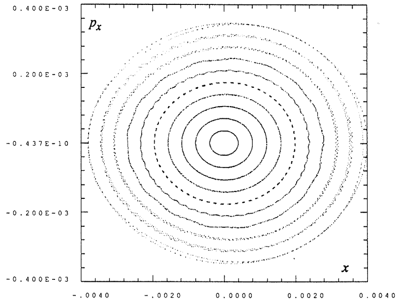
FIGURE 17.18. This figure shows, for the ALS, tracking results in the (x, p_x) plane for 1000 iterations of a Cremona symplectification \mathcal{C}_5^{cub} of the fourth-order truncated Taylor map \mathcal{T}_5 using the same initial conditions employed in Figure 17.15. In this case the \mathcal{L}_j were based on the fifth-order, twelve-point cubature formula for the two-sphere.
