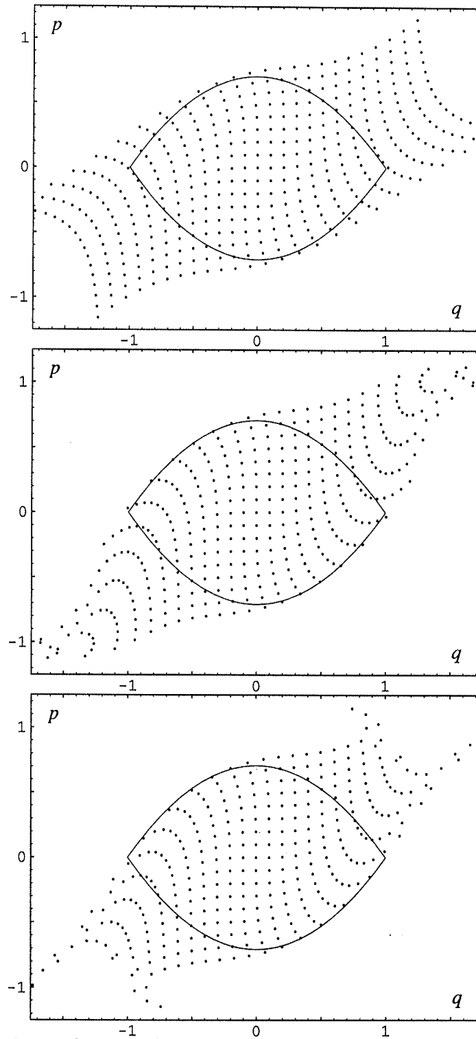
FIGURE 17.4. These graphics show for the anharmonic oscillator the results of applying once to the initial conditions shown in Figure 17.1 the non-linear part of the Cremona maps \mathcal{C}_4 (top), \mathcal{C}_8 (middle), and \mathcal{C}_{12} (bottom) obtained by Cremona symplectification of the corresponding truncated Taylor maps \mathcal{T}_4 , \mathcal{T}_8 , and \mathcal{T}_{12} for time \tau = 1 .
