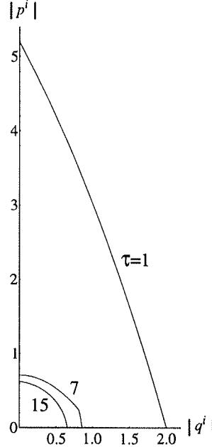
FIGURE 6.6. This graph shows the DAC boundaries for the Taylor series map at three different time steps: \tau = 1, 7 , and 15 . The boundary for \tau = 1 lies well outside the separatrix. For \tau = 7 , a relatively long time step, part of the boundary lies right next to the separatrix, while the rest of the boundary cuts inside the separatrix. And for \tau = 15 all of the boundary lies inside the separatrix.
