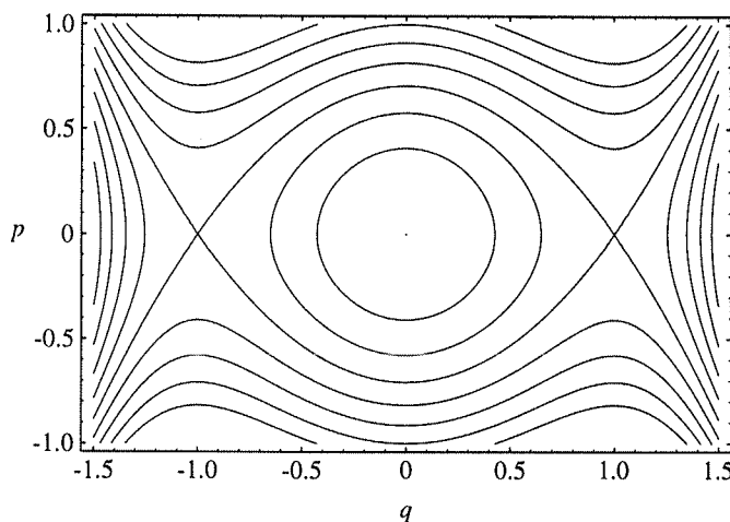
FIGURE 6.2. Phase-space portrait of the quartic anharmonic oscillator.
