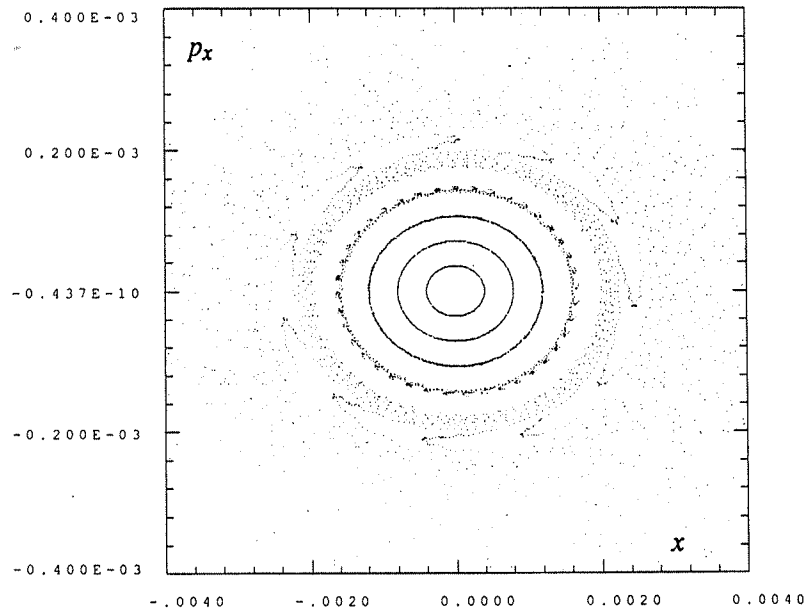
FIGURE 17.16. This figure shows, for the ALS, tracking results in the (x, p_x) plane for 1000 iterations of a fourth-order truncated Taylor map \mathcal{T}_5 using the same initial conditions employed in Figure 17.15.
