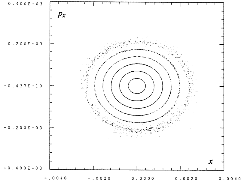
FIGURE 17.17. This figure shows, for the ALS, tracking results in the (x, p_x) plane for 1000 iterations of a Cremona symplectification \mathcal{C}_5^{rand} of the fourth-order truncated Taylor map \mathcal{T}_5 using the same initial conditions employed in Figure 17.15. In this case the \mathcal{L}_j were chosen randomly.
