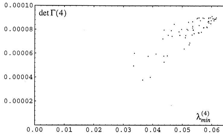
FIGURE 16.5. This plot shows the determinant \det \Gamma(4) versus the minimum eigenvalue \lambda_{min}^{(4)} for sixty-four different Gram matrices obtained using a genetic algorithm with a fitness function given by \lambda_{min}^{(4)} . (See the text for more details.)
