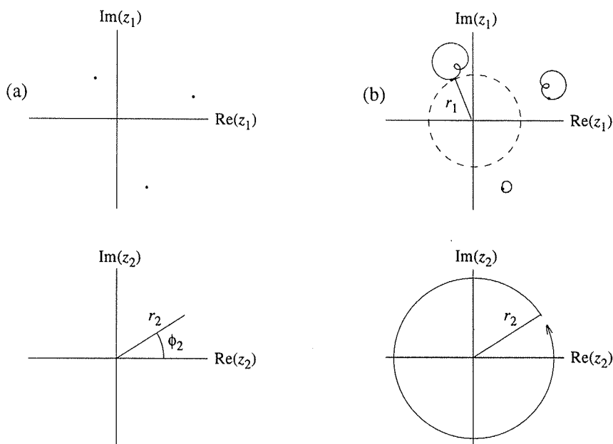
FIGURE 4.2. Computing the domain of absolute convergence. We sketch here a possible scenario for a function F(z_1, z_2) whose only singularities are poles. The upper pair of graphs represents the complex z_1 -plane, while the lower pair represents the complex z_2 -plane. For a fixed value of z_2 = r_2 e^{i\phi_2} , the function F(z_1, z_2) might have singularities near the origin as shown on the left in (a). As the phase \phi_2 of z_2 sweeps through an interval of 2\pi , the singularities in the z_1 -plane trace out closed curves, as shown on the right in (b).
