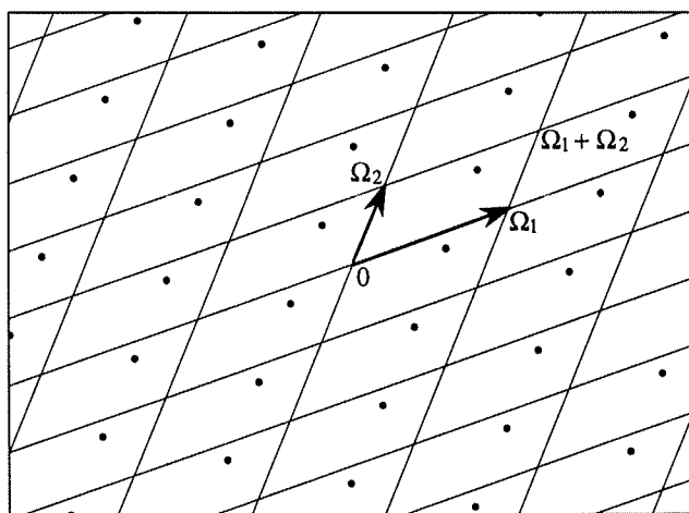
FIGURE A.2. A lattice of points ( \cdot ) congruent with respect to the periods \Omega_1 and \Omega_2 .
