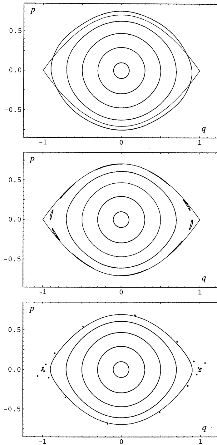
FIGURE 17.9. These graphics show for the anharmonic oscillator tracking results obtained from 1000 iterations of the Cremona maps C_4 (top), C_8 (middle), and C_{12} (bottom) for time \tau = 1 using the initial conditions p^i = 0 , q^i \in \{\pm 0.1, \pm 0.3, \pm 0.5, \pm 0.7, \pm 0.9\} . The bottom figure also uses the initial conditions (q^i, p^i) = (1.0, -0.2) and (q^i, p^i) = (-1.0, 0.2) .
