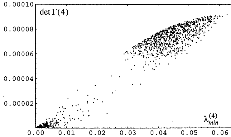
FIGURE 16.4. This plot combines the results shown in Figures 16.1 and 16.3.
