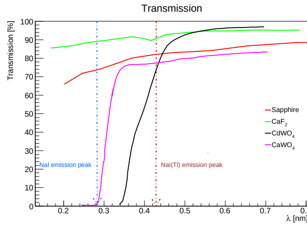
Figure 6.3.3: Crystal light transmission as a function of the wavelength for \text{CdWO}_4 (black) [260], sapphire (red), \text{CaF}_2 (green) [261] and \text{CaWO}_4 (magenta) [262]. For pure NaI and NaI(Tl) in addition the peaks of the scintillation light emission are shown, see [263].
