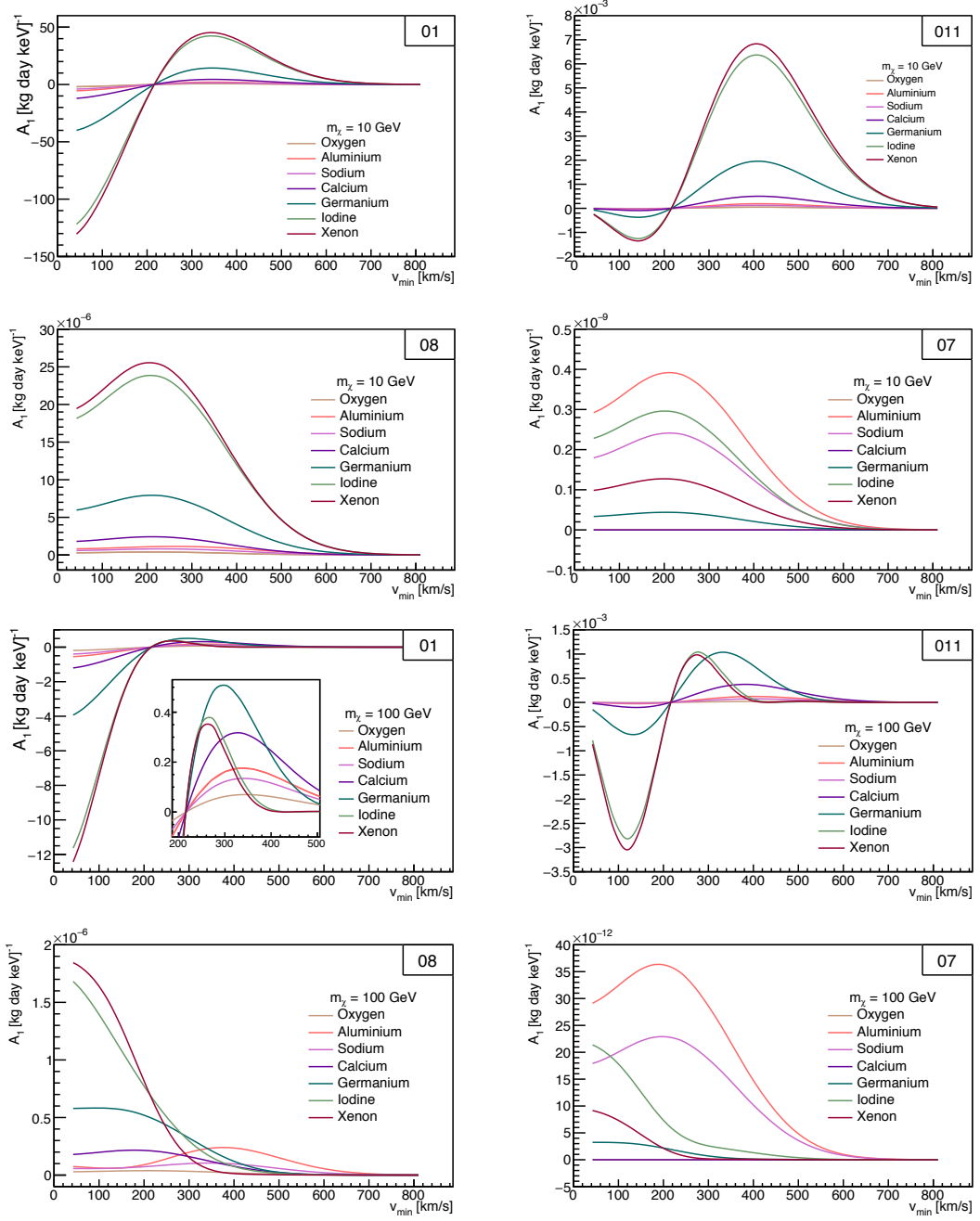
Figure 4.2.2: Top: Amplitude of modulation for the four non-relativistic effective operators \hat{\mathcal{O}}_1 , \hat{\mathcal{O}}_7 , \hat{\mathcal{O}}_8 , \hat{\mathcal{O}}_{11} and m_\chi = 10 GeV. Different colours correspond to different targets. The effective coupling constants are fixed at c_0^i = 1/246 GeV 2 . Bottom: Same as on top plot, but with m_\chi = 100 GeV. This selection of operators includes interactions with different dependency on the relative DM-nucleon velocity.
