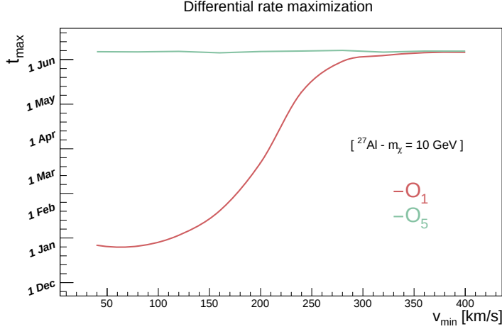
Figure 4.2.3: Time of maximal rate during the year plotted as function of the minimal velocity, for the effective operators \hat{\mathcal{O}}_1 and \hat{\mathcal{O}}_5 , for aluminium and m_\chi = 10 GeV.
