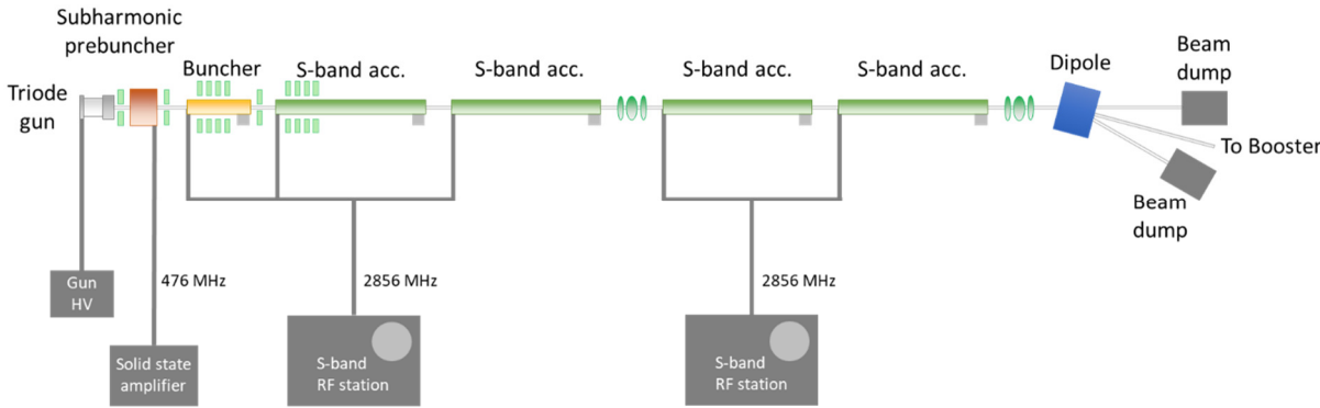
Figure 2: Configuration of the SPS-II injector linac.
