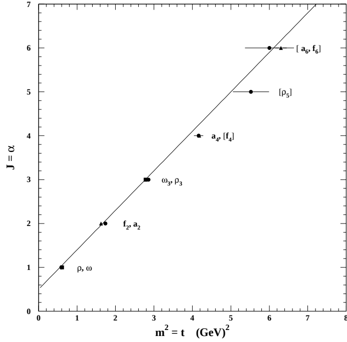
Figure 2.2: The \rho , \omega , f and a trajectories.
