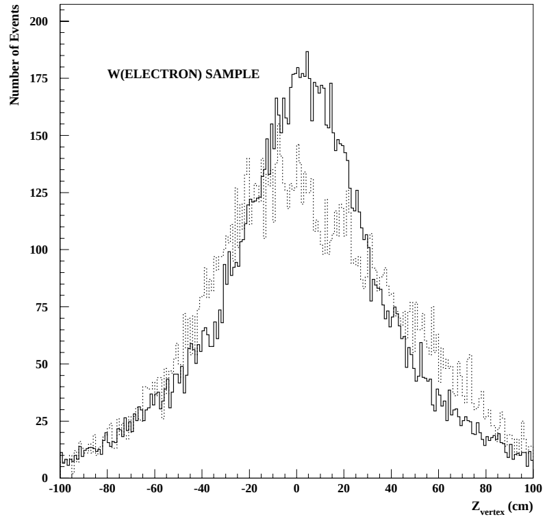
Figure 6.1: z_{\text{vertex}} -distribution for W (central electron) events from run 1B: (dotted line) events from 55267 < \text{run \#} < 61739 ; (solid line) events from 61739 < \text{run \#} < 71023 .
