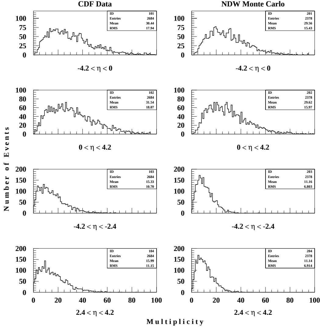
Figure 6.8: Data (towers) and non-diffractive Monte Carlo (particles) multiplicity distributions.
