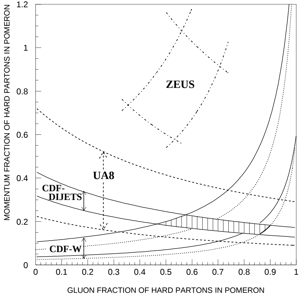
Figure 7.1: Momentum fraction versus gluon fraction of hard partons in the pomeron evaluated by comparing measured diffractive rates with MC predictions based on the standard (see text) pomeron flux and assuming that only hard partons in the pomeron participate in the diffractive process considered. Results are shown for ZEUS (dashed-dotted), UA8 (dashed) and the CDF-DIJETS and CDF-W measurements. The CDF-W result is shown for two (dotted) or three (solid) light quark flavors in the pomeron. The shaded region is used in the text to extract the quark to gluon fraction of the pomeron and the standard flux discrepancy factor.
