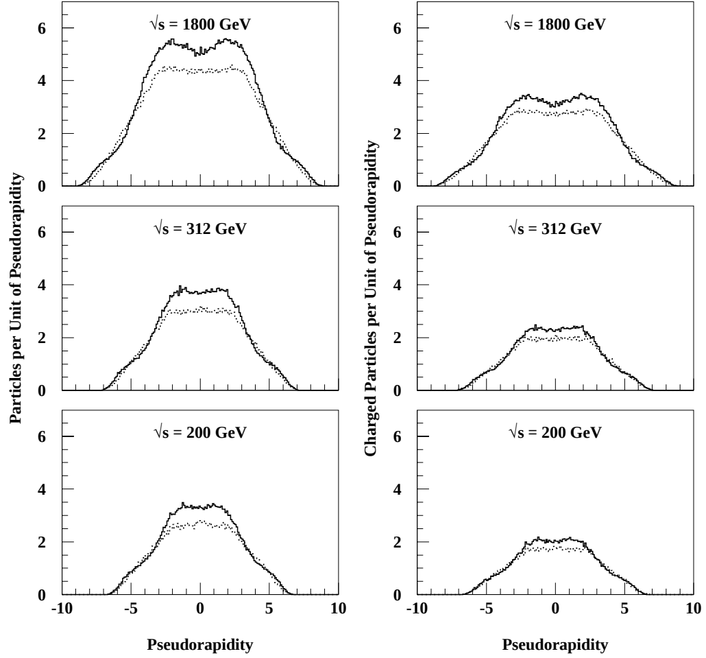
Figure 5.1: Total (left) and charged (right) particle dn/d\eta distributions for PYTHIA (solid) and MBR (dotted) minimum bias events.
