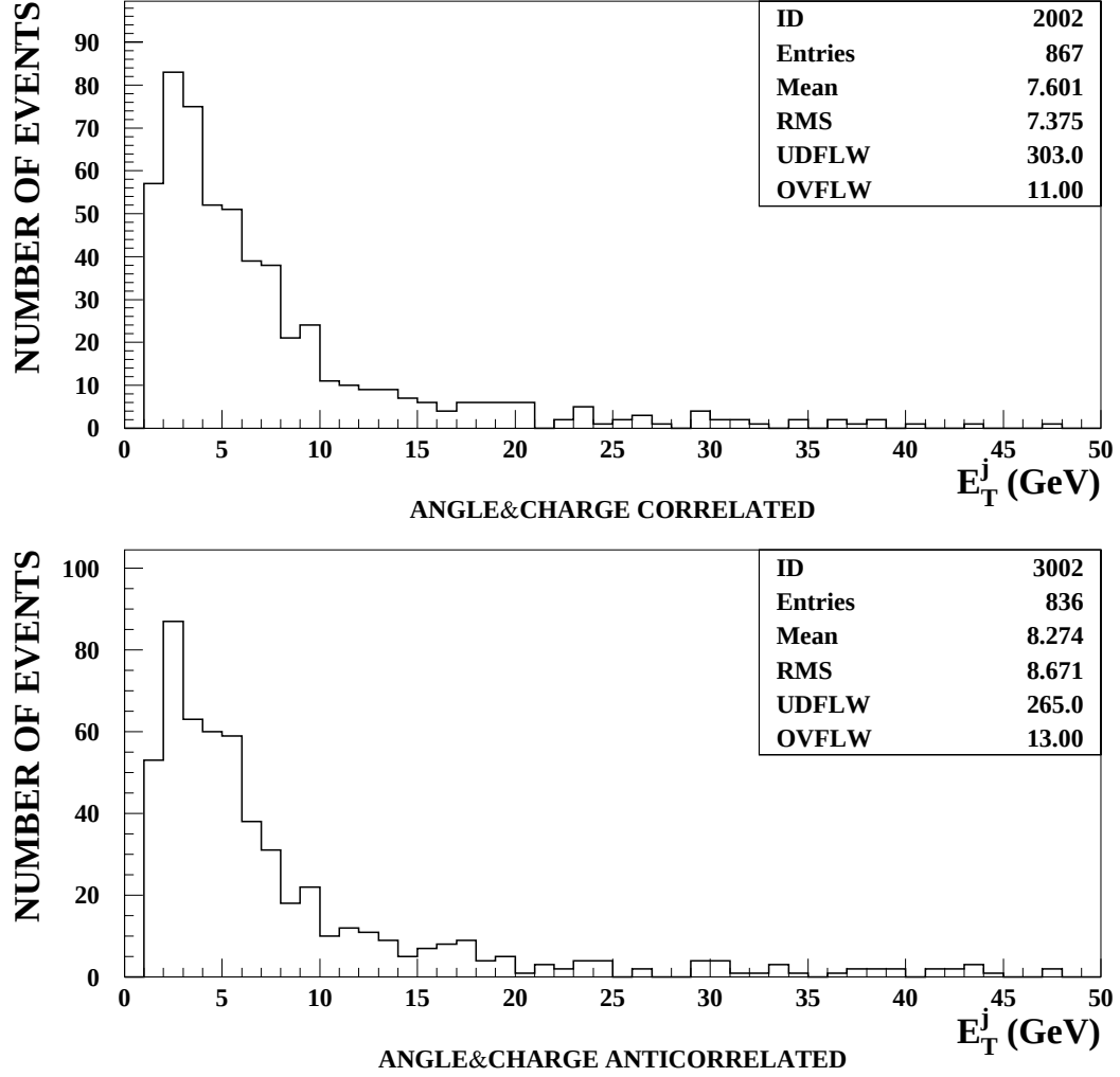
Figure 6.29: Jet E_T distributions for (angle \otimes charge)-correlated (top) and (angle \otimes charge)-anticorrelated (bottom) data W events in the control sample.
