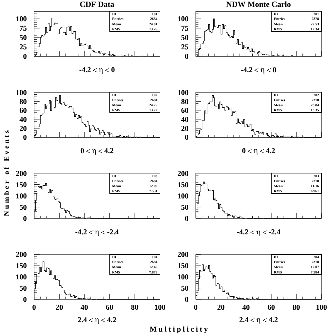
Figure 6.15: Multiplicity distributions for data (tower clusters) and MC (particles) after P_T correction.
