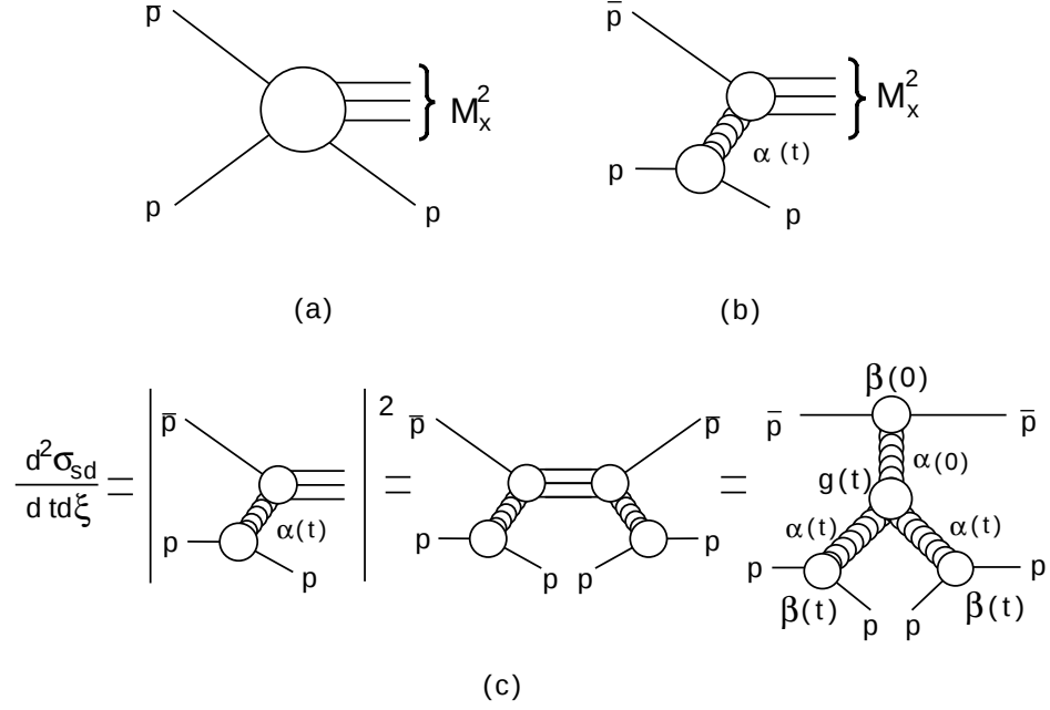
Figure 2.5: (a) Pseudo two-body amplitude of inelastic diffraction. (b) Regge approximation of the amplitude for large s , small \xi , and t \ll s . (c) Triple Regge diagram of differential single diffraction cross section.
