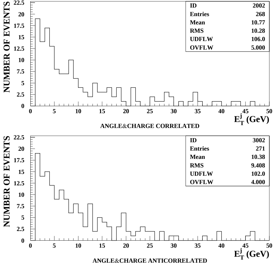
Figure 6.32: Jet E_T distributions for (angle \otimes charge) -correlated (top) and (angle \otimes charge) -anticorrelated (bottom) non-diffractive W Monte Carlo events in the signal region.
