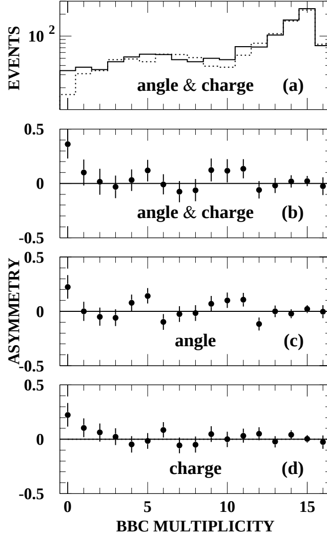
Figure 6.18: Electron angle and/or charge correlated and anticorrelated distributions (see text) versus BBC multiplicity. In each case shown the asymmetry is defined as the bin-by-bin difference over the sum of the correlated and anticorrelated distributions.
