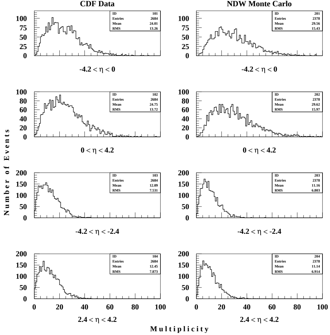
Figure 6.10: Data (tower clusters) and non-diffractive MC (particles) multiplicity distributions.
