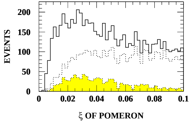
Figure 6.28: Pomeron \xi -distribution for all Monte Carlo generated diffractive W events (solid line), for events with a central electron/positron (dotted line), and for events with a central electron/positron which are (angle \otimes charge)-correlated with a BBC of multiplicity zero, one or two hits and N_{\text{towers}} < 8 (shaded histogram).
