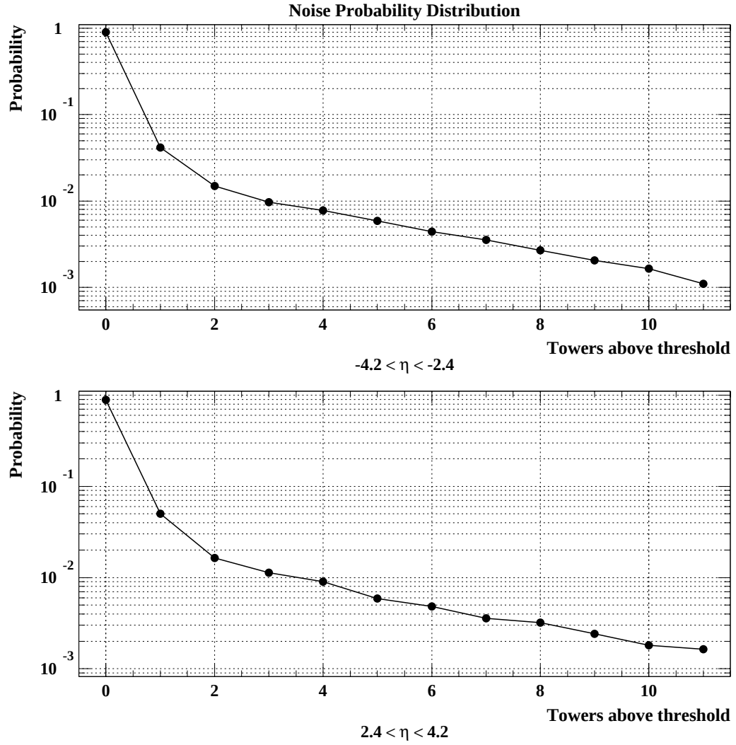
Figure 6.6: The probability distribution for the number of towers above the E_T threshold in the regions -4.2 < \eta < -2.4 and 2.4 < \eta < 4.2 for the beam-beam crossing event sample.
