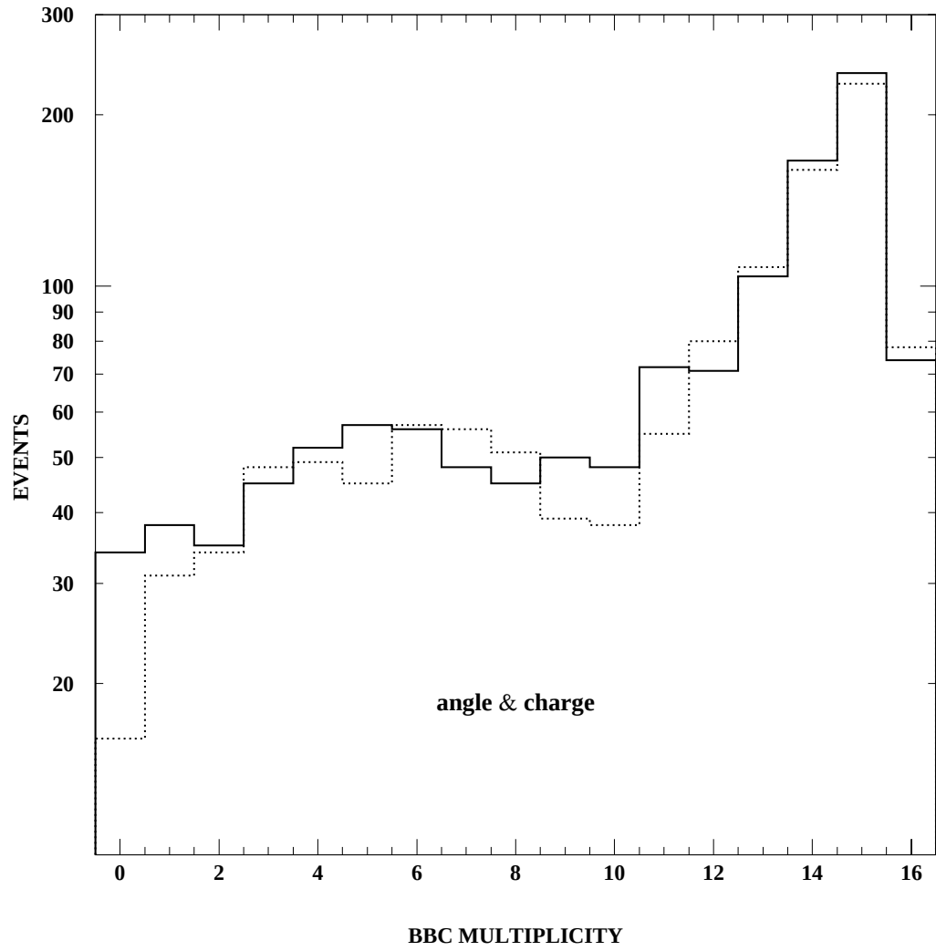
Figure 6.19: Electron angle-gap and charge-gap doubly-correlated (solid) and anticorrelated (dashed) distributions versus BBC multiplicity.
