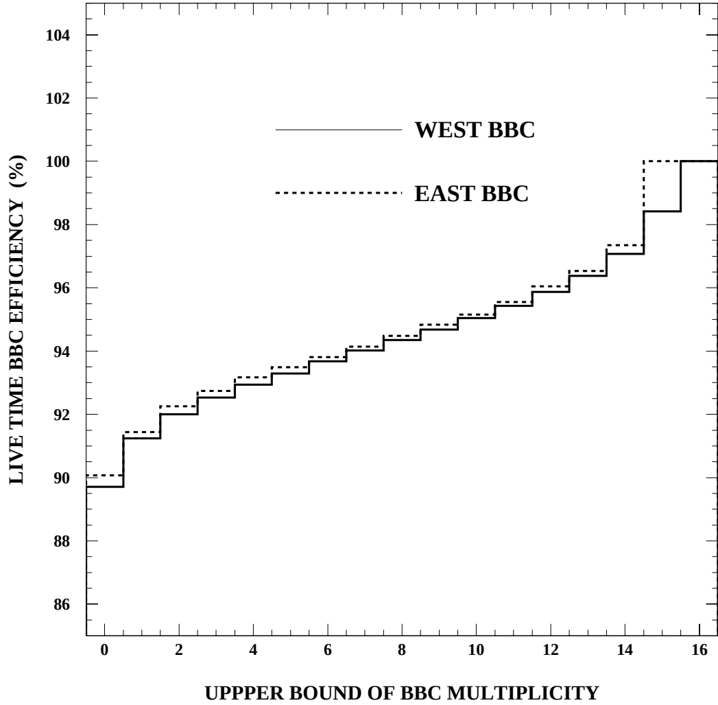
Figure 6.27: The BBC livetime efficiency as a function of the upper bound of BBC multiplicity, N_B , for the run 1A data.
