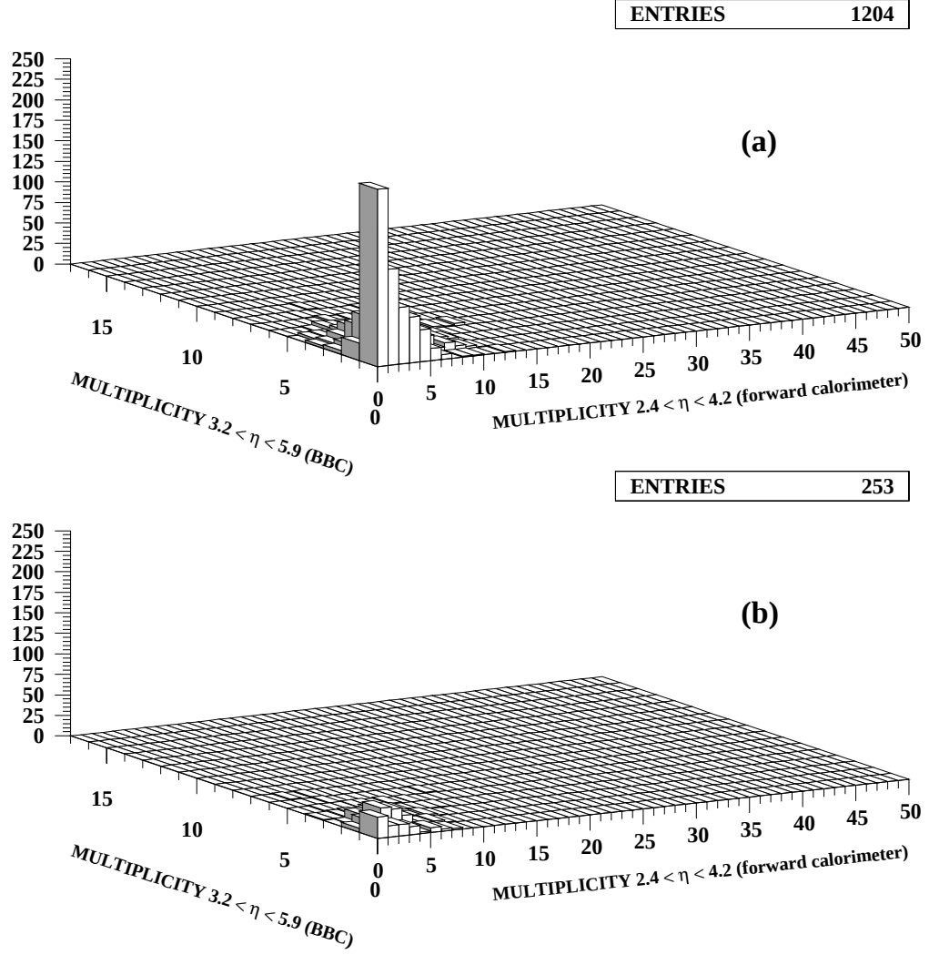
Figure 6.25: Multiplicity of particles in the pseudorapidity region 2.4 < \eta < 4.2 (forward calorimeter) and in the adjacent BBC region 3.2 < \eta < 5.9 (a) for (angle \otimes charge)-correlated and (b) for (angle \otimes charge)-anticorrelated diffractive W events generated with POMPYT using a hard-quark structure for the pomeron.
