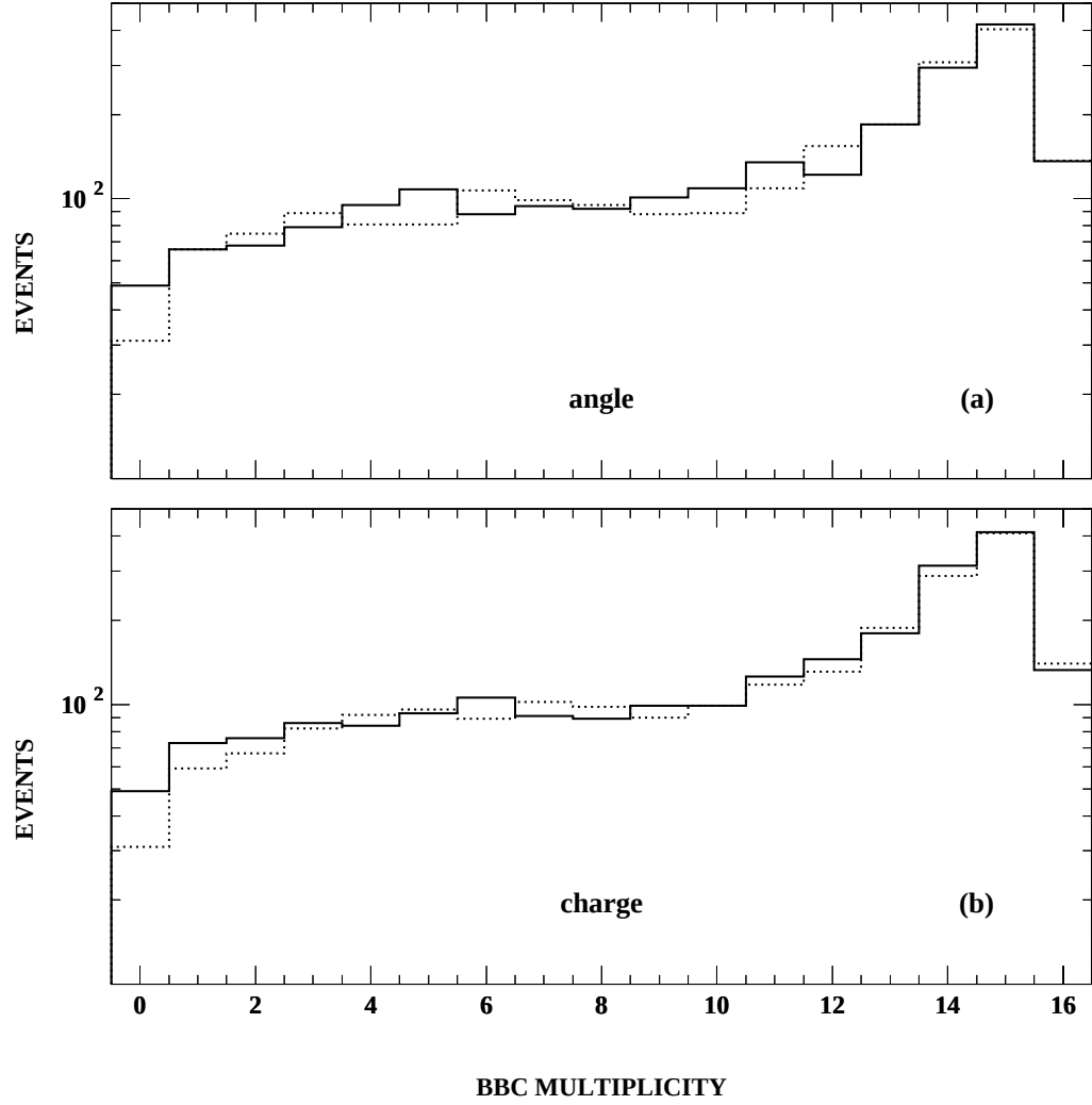
Figure 6.21: Electron angle-gap and charge-gap correlated (solid) and anticorrelated (dashed) distributions versus BBC multiplicity.
