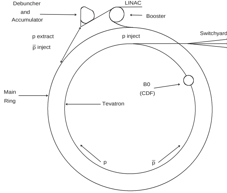
Figure 4.1: Schematic view of the Fermilab p\bar{p} collider.
