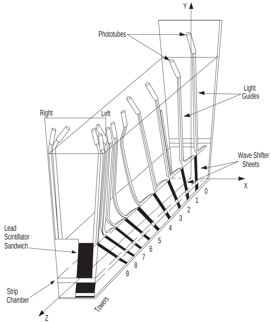
Figure 4.6: Layout of the CEM light-gathering system in a single wedge of the CEM and CHA calorimeters.
