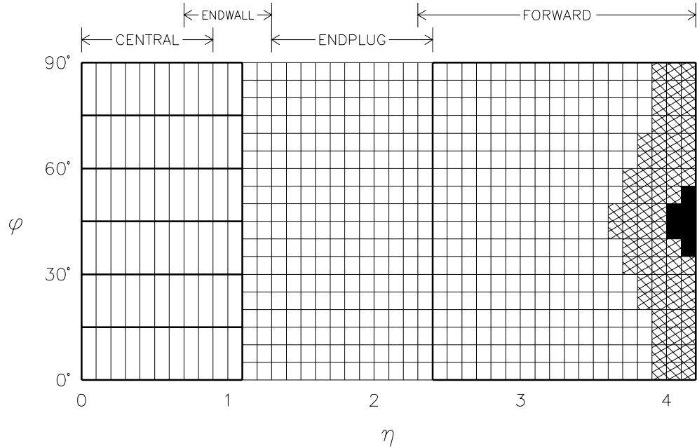
Figure 4.5: Schematic \eta - \phi segmentation of the CDF calorimeters. The shaded region represents partial depth coverage to accommodate the low- \beta quadrupole magnets; the black region has no calorimetric coverage.
