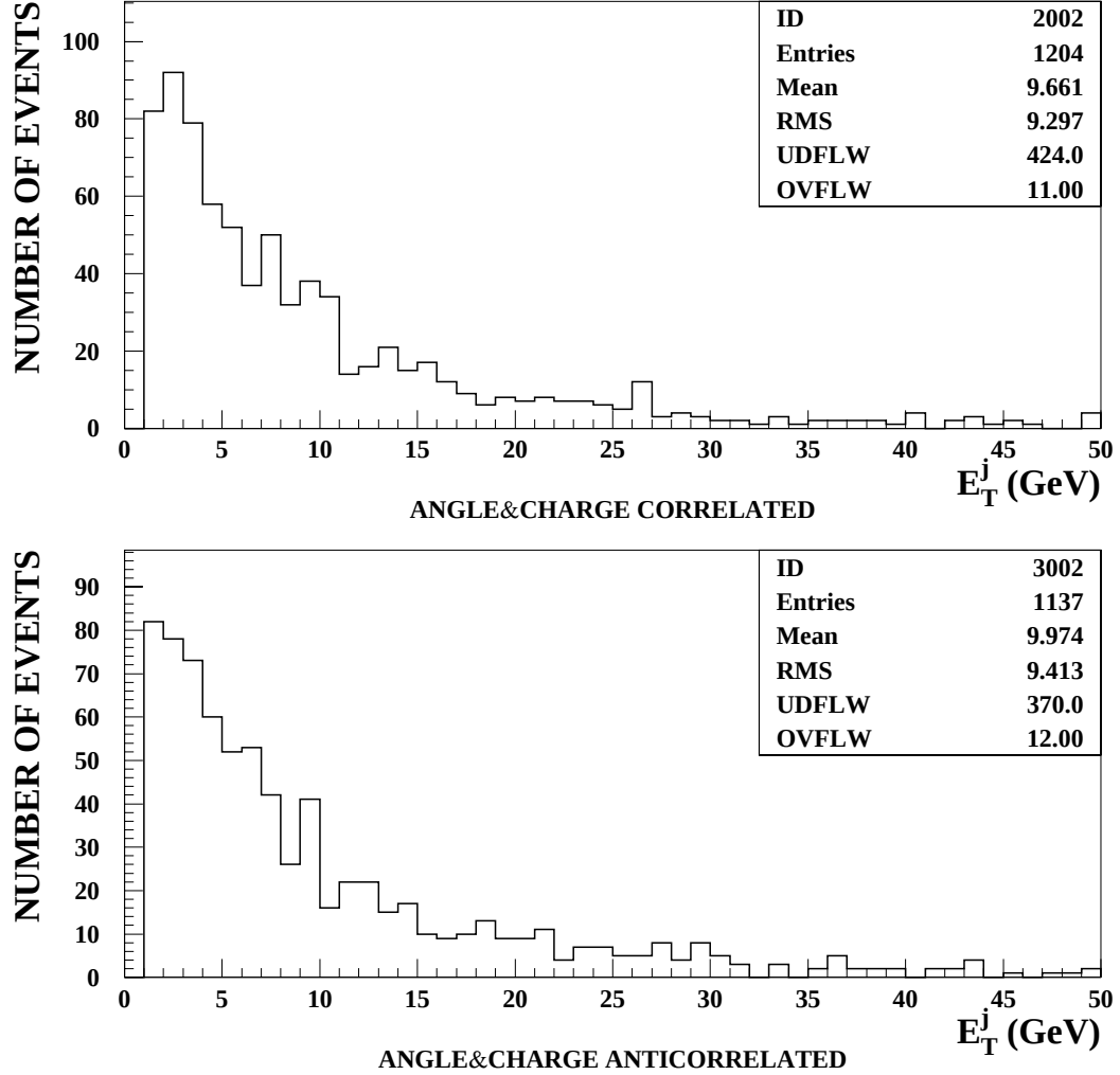
Figure 6.30: Jet E_T distributions for (angle⊗charge)-correlated (top) and (angle⊗charge)-anticorrelated (bottom) non-diffractive W Monte Carlo events in the control sample.
