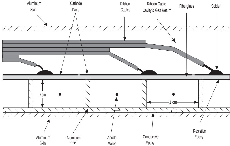
Figure 4.7: Cross section of a FEM chamber.
