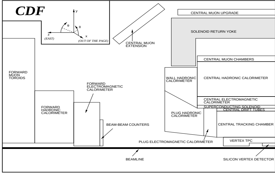
Figure 4.3: Schematic side-view cross section of 1/4 of the CDF detector displaying main detector components.
