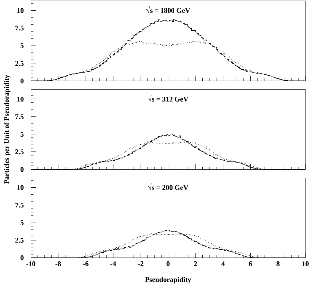
Figure 5.2: Comparison of the dn/d\eta distributions for the underlying event in W -boson production (solid), and for minimum bias events (dotted), simulated with the PYTHIA Monte Carlo program for \bar{p}p collisions at 200, 312 and 1800 GeV.
