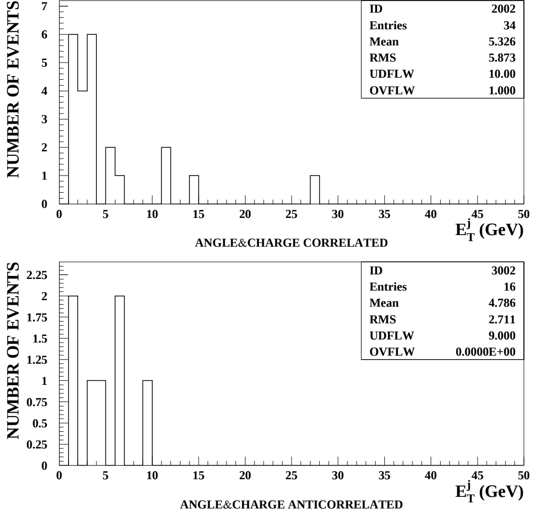
Figure 6.31: Jet E_T distributions for (angle \otimes charge)-correlated (top) and (angle \otimes charge)-anticorrelated (bottom) data W events in the signal region.
