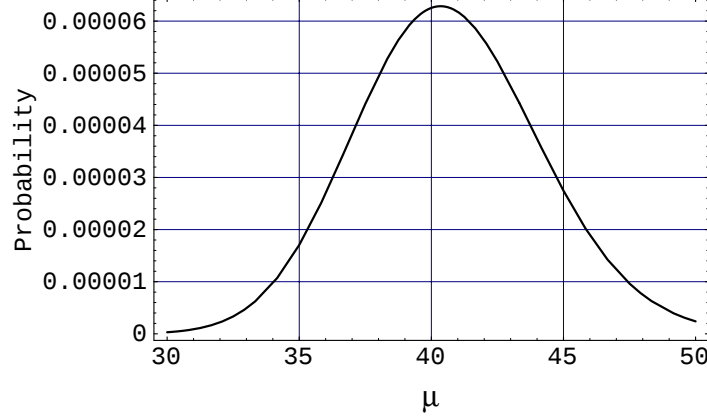
Figure 6.22: Probability versus \mu for angle and charge (anti)correlated events.
