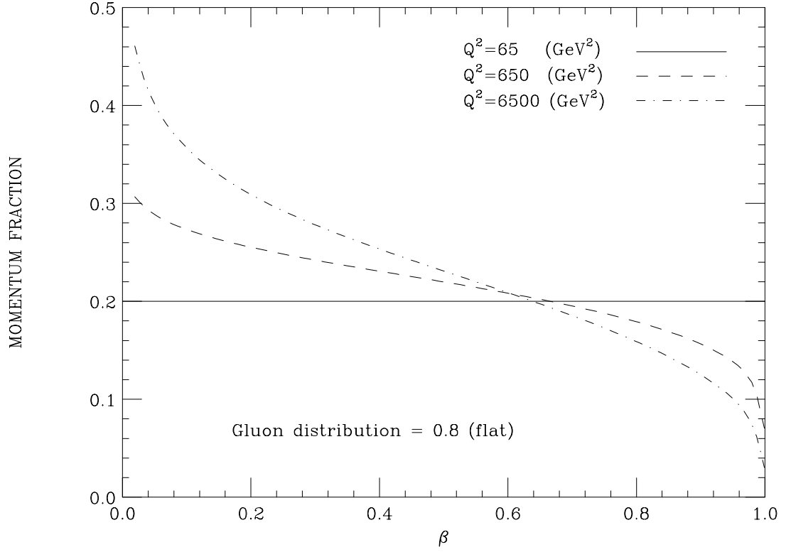
Figure 7.2: Effect of DGLAP Q^2 evolution on the quark component of the pomeron structure. (solid line) input quark distribution, taken to be flat in \beta at Q^s=65 GeV 2 ; (dashed line) quark distribution at Q^2=650 GeV 2 ; (dashed-dotted line) quark distribution at Q^2=6500 GeV 2 .
