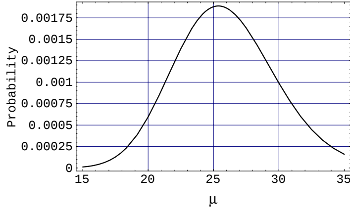
Figure 6.20: Probability versus \mu for (angle \otimes charge)-(anti)correlated events.
