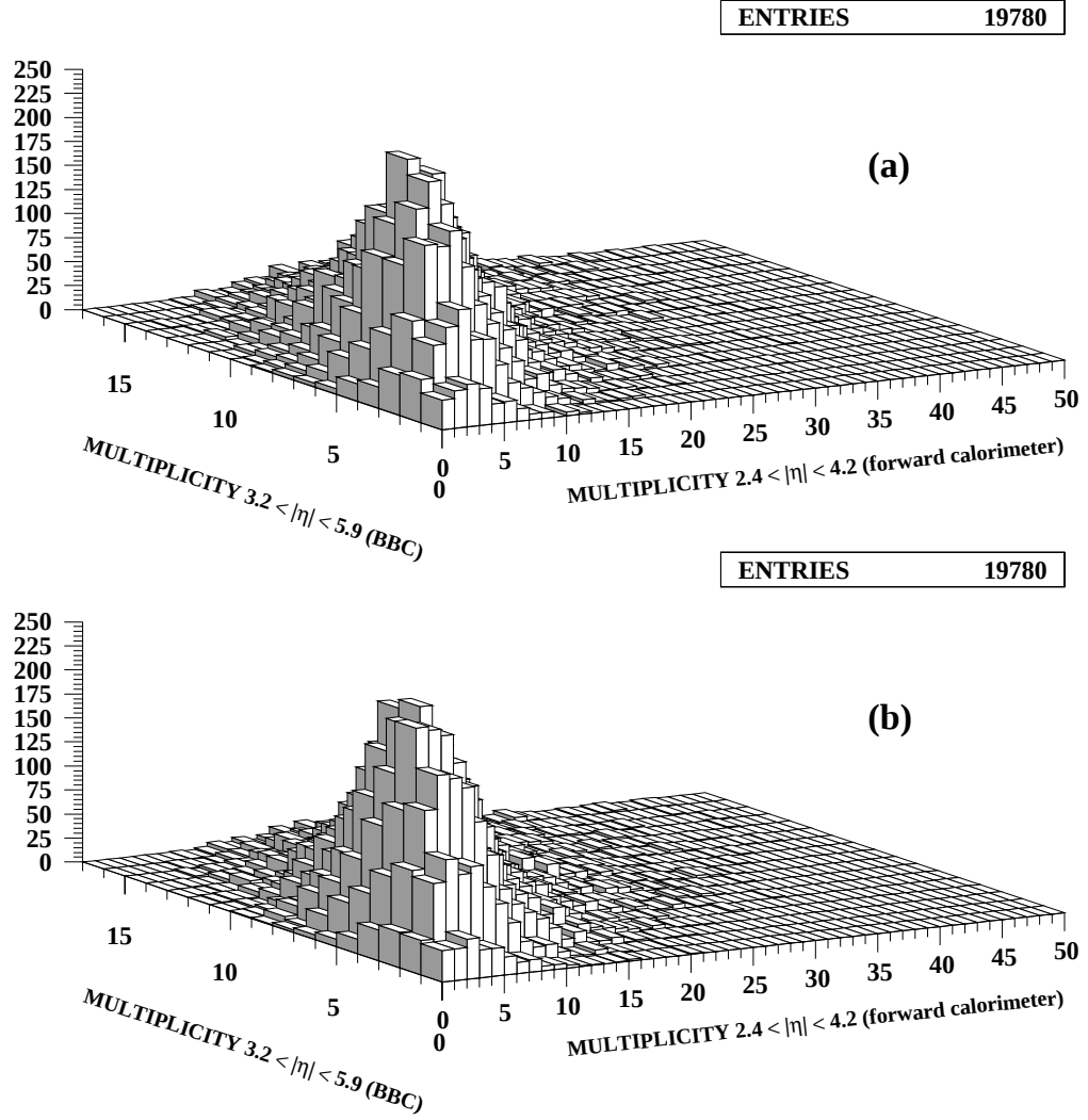
Figure 6.26: Multiplicity of particles in the pseudorapidity region 2.4 < |\eta| < 4.2 (forward calorimeter) and in the adjacent BBC region 3.2 < |\eta| < 5.9 (a) for (\text{angle} \otimes \text{charge}) -correlated and (b) for (\text{angle} \otimes \text{charge}) -anticorrelated (b) non-diffractive W events generated with PYTHIA.
