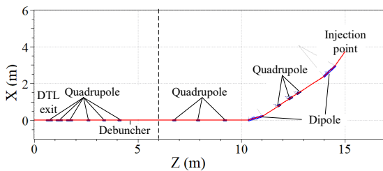
Figure 6: Layout of the main components of LRBT.
