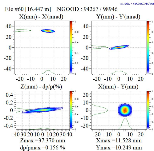
Figure 8: Beam phase spaces at the exit of injection point.
