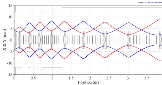
Figure 5: 2.45 times RMS beam envelope in the IH-DTL.
