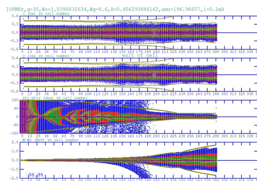
Figure 4: Beam dynamics in the RFQ (from top to bottom: envelope in x direction; envelope in y direction; envelope in phase; envelope in energy).
