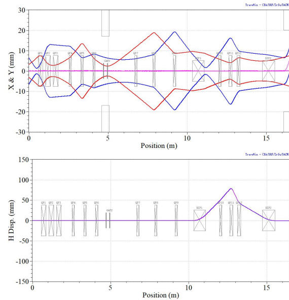
Figure 7: Beam dynamics in the LRBT (top: 2.45 times RMS beam envelope; bottom: horizontal dispersion).
