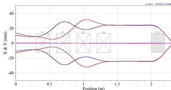
Figure 3: 2.45 times RMS beam envelope in the LEBT.
