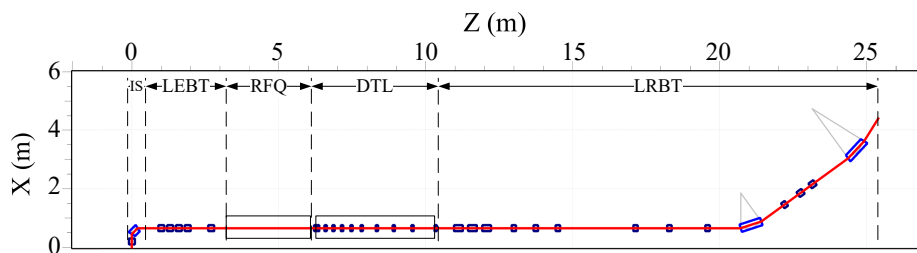
Figure 1: Sketch of the whole injector.
