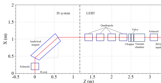
Figure 2: Sketch of the ion source system and the LEBT.
