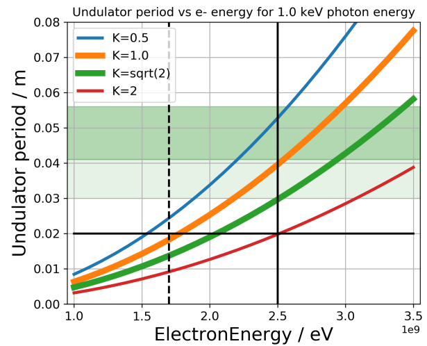
Figure 2: The choice of the beam energy depending on the undulator period selection for different K . Main period length of APPLE II used at BESSY II are indicated with the dark green area and could be extended towards the light green area by closing the gap to minimum values of 9 mm.
