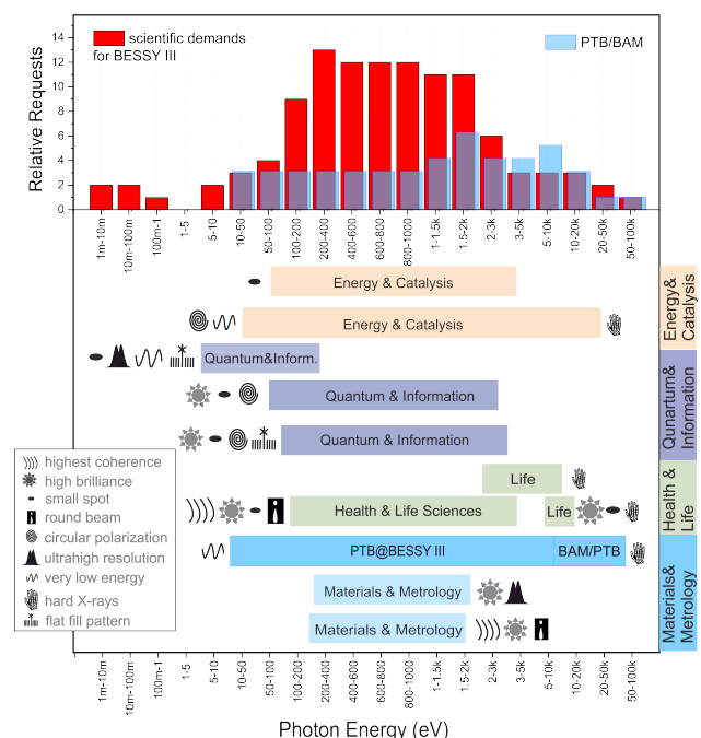
Figure 1: Main demands and requirements on BESSY III.
